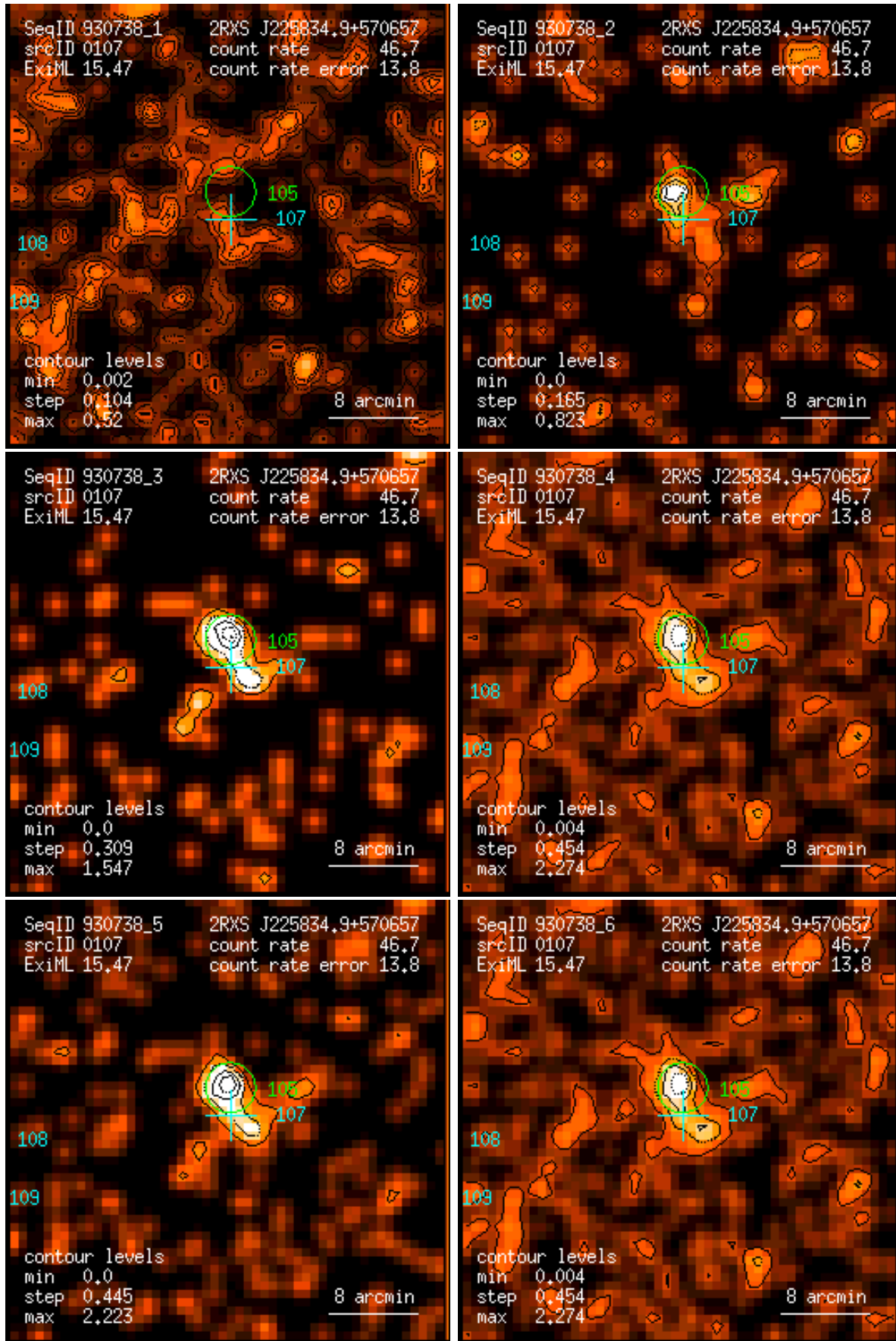
Figure 107: RASS 930738: detection 0107: band rate images, Gaussian filter: (1) PSPC channels 11 – 41, (2) 52 – 90, (3) 91 – 201, (4) 11 – 235, (5) 52 – 201, (6) 11 – 201. Broad band rates in counts/ks. Band rate contour levels in counts/ks/arcmin 2 .
