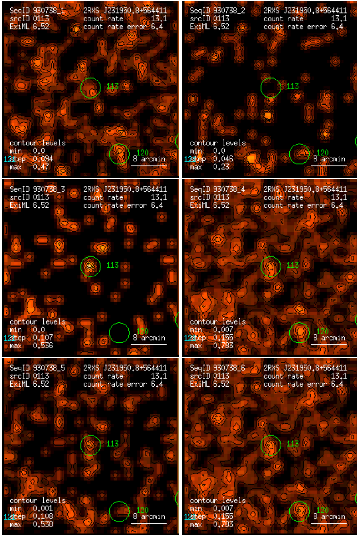
Figure 113: RASS 930738: detection 0113: band rate images, Gaussian filter: (1) PSPC channels 11 – 41, (2) 52 – 90, (3) 91 – 201, (4) 11 – 235, (5) 52 – 201, (6) 11 – 201. Broad band rates in counts/ks. Band rate contour levels in counts/ks/arcmin 2 .
