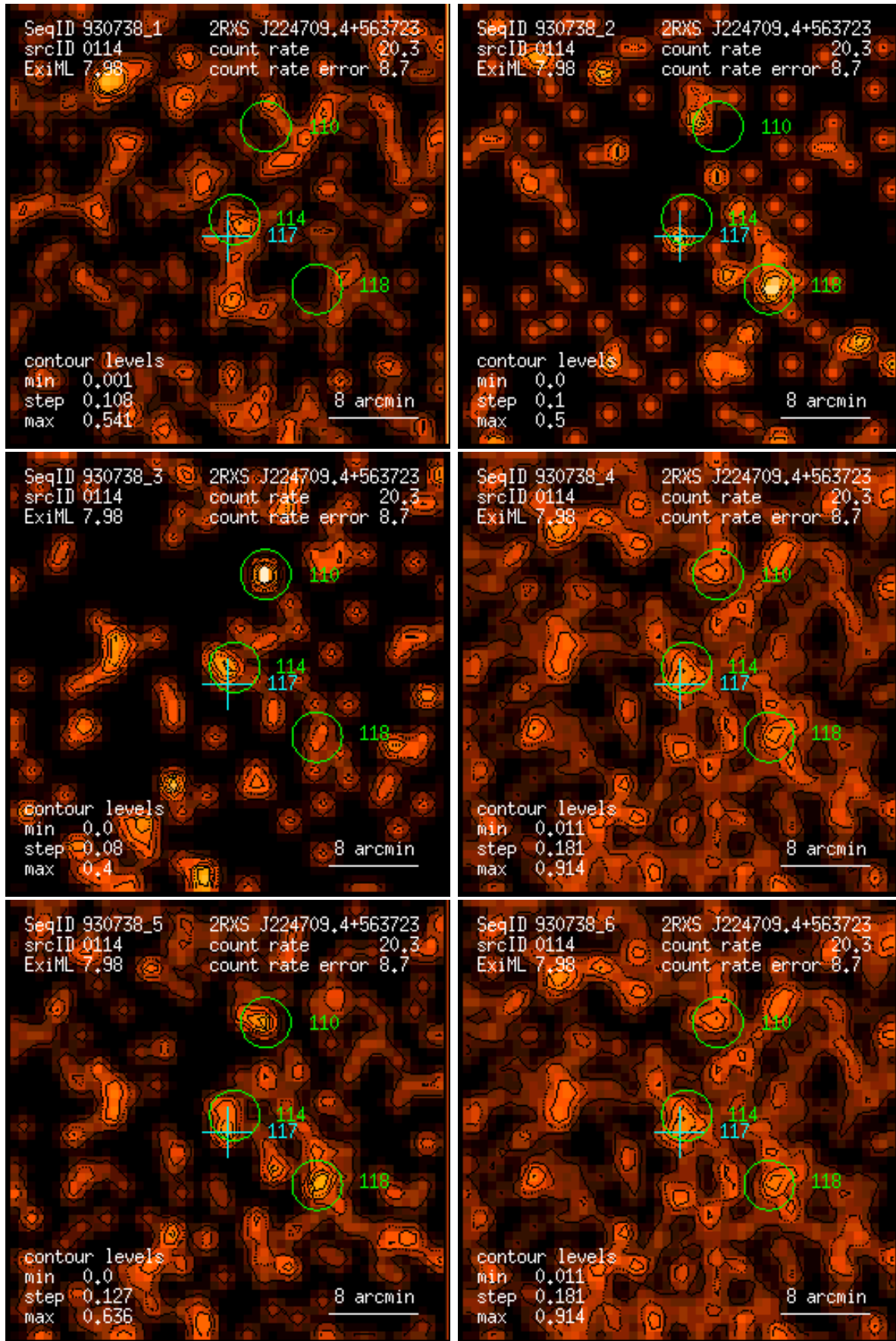
Figure 114: RASS 930738: detection 0114: band rate images, Gaussian filter: (1) PSPC channels 11 – 41, (2) 52 – 90, (3) 91 – 201, (4) 11 – 235, (5) 52 – 201, (6) 11 – 201. Broad band rates in counts/ks. Band rate contour levels in counts/ks/arcmin 2 .
