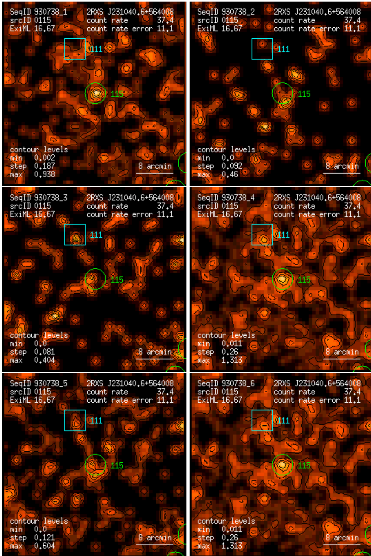
Figure 115: RASS 930738: detection 0115: band rate images, Gaussian filter: (1) PSPC channels 11 – 41, (2) 52 – 90, (3) 91 – 201, (4) 11 – 235, (5) 52 – 201, (6) 11 – 201. Broad band rates in counts/ks. Band rate contour levels in counts/ks/arcmin 2 .
