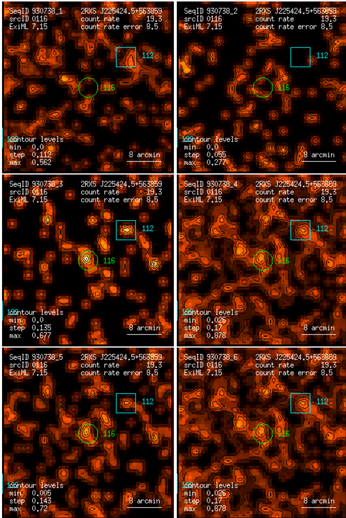
Figure 116: RASS 930738: detection 0116: band rate images, Gaussian filter: (1) PSPC channels 11 – 41, (2) 52 – 90, (3) 91 – 201, (4) 11 – 235, (5) 52 – 201, (6) 11 – 201. Broad band rates in counts/ks. Band rate contour levels in counts/ks/arcmin 2 .
