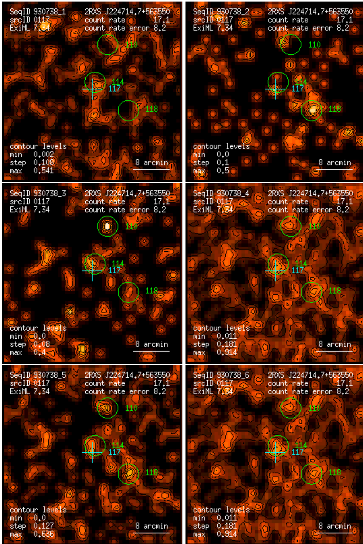
Figure 117: RASS 930738: detection 0117: band rate images, Gaussian filter: (1) PSPC channels 11 – 41, (2) 52 – 90, (3) 91 – 201, (4) 11 – 235, (5) 52 – 201, (6) 11 – 201. Broad band rates in counts/ks. Band rate contour levels in counts/ks/arcmin 2 .
