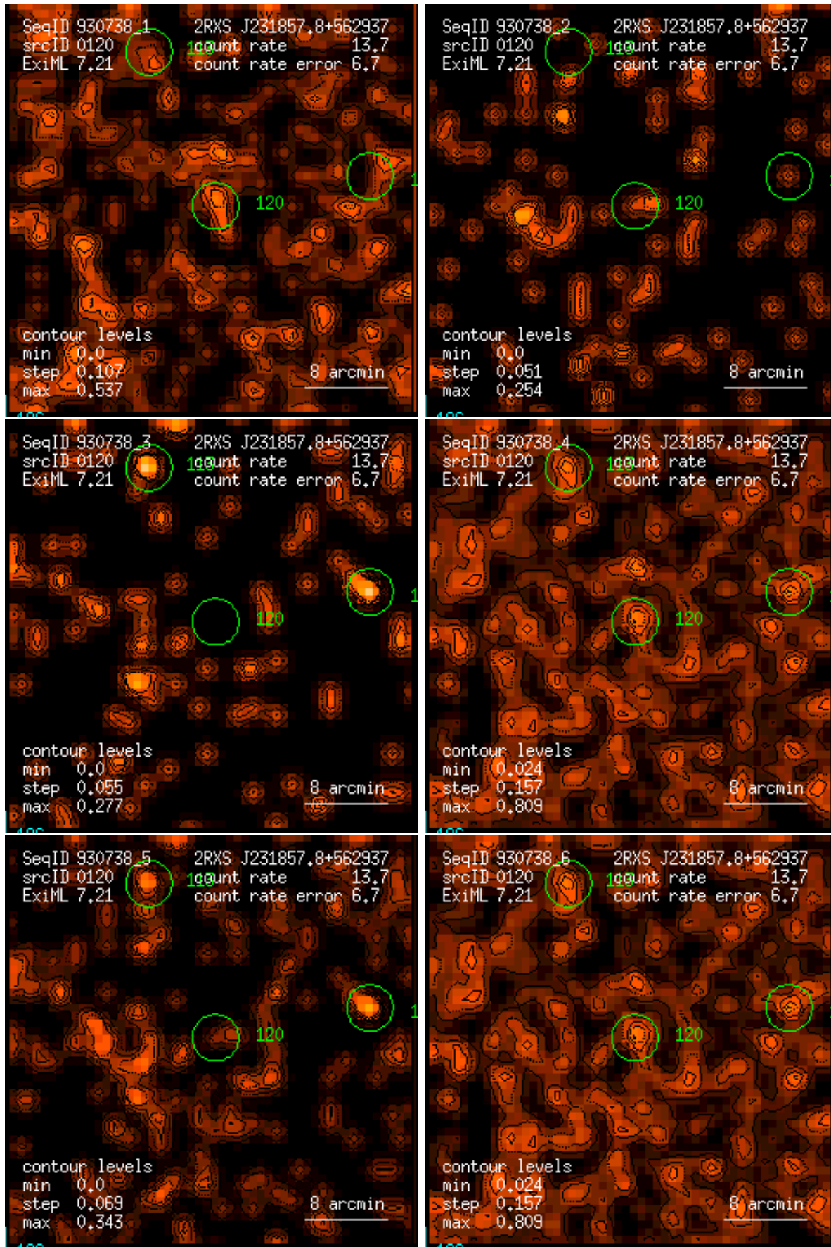
Figure 120: RASS 930738: detection 0120: band rate images, Gaussian filter: (1) PSPC channels 11 – 41, (2) 52 – 90, (3) 91 – 201, (4) 11 – 235, (5) 52 – 201, (6) 11 – 201. Broad band rates in counts/ks. Band rate contour levels in counts/ks/arcmin 2 .
