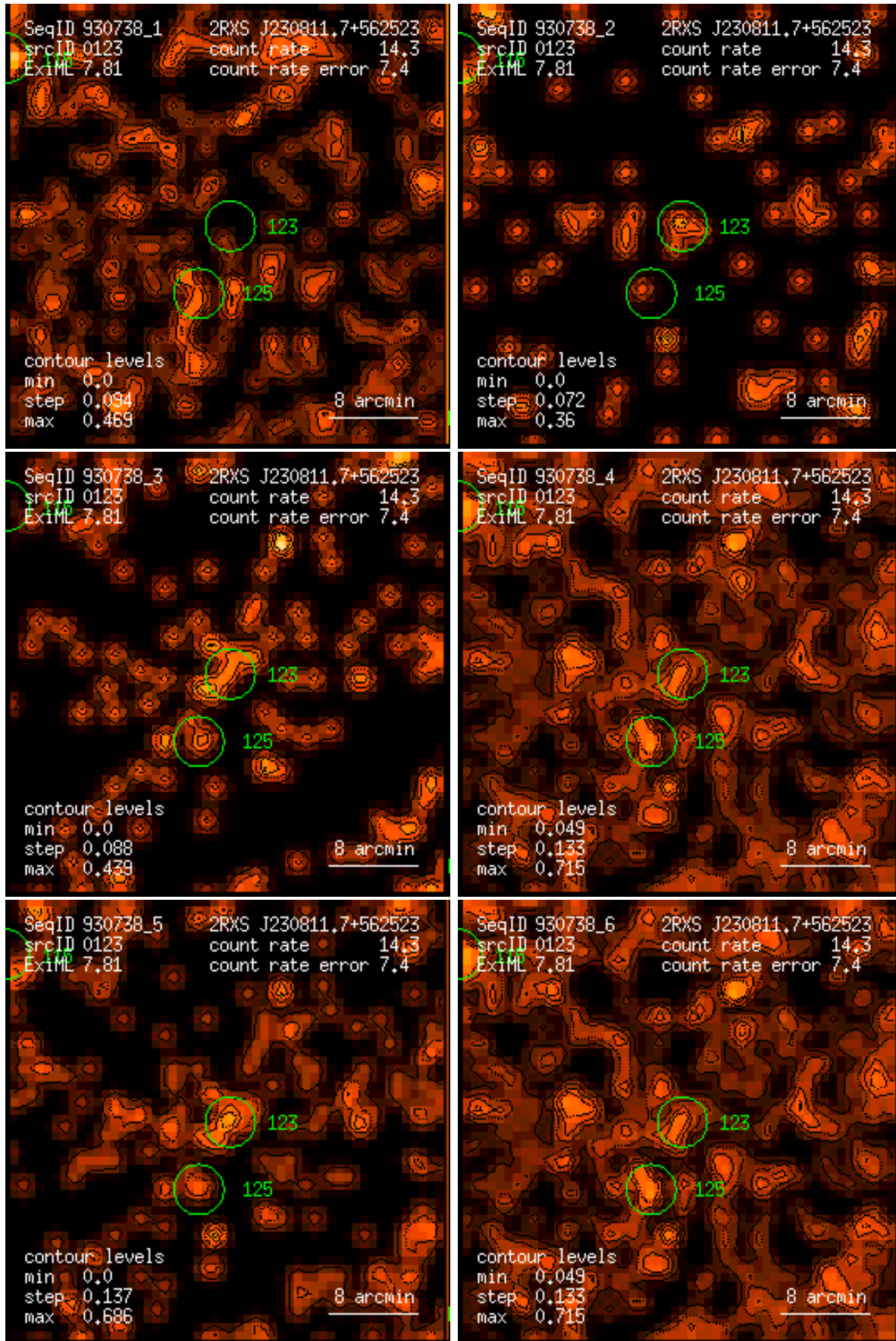
Figure 123: RASS 930738: detection 0123: band rate images, Gaussian filter: (1) PSPC channels 11 – 41, (2) 52 – 90, (3) 91 – 201, (4) 11 – 235, (5) 52 – 201, (6) 11 – 201. Broad band rates in counts/ks. Band rate contour levels in counts/ks/arcmin 2 .
