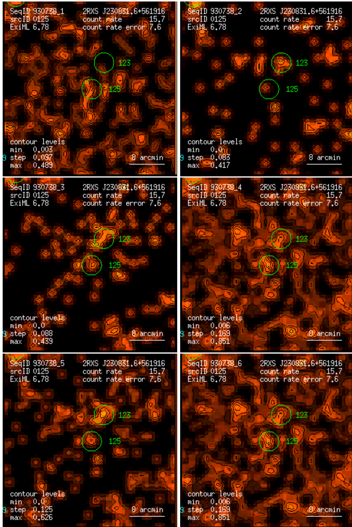
Figure 125: RASS 930738: detection 0125: band rate images, Gaussian filter: (1) PSPC channels 11 – 41, (2) 52 – 90, (3) 91 – 201, (4) 11 – 235, (5) 52 – 201, (6) 11 – 201. Broad band rates in counts/ks. Band rate contour levels in counts/ks/arcmin 2 .
