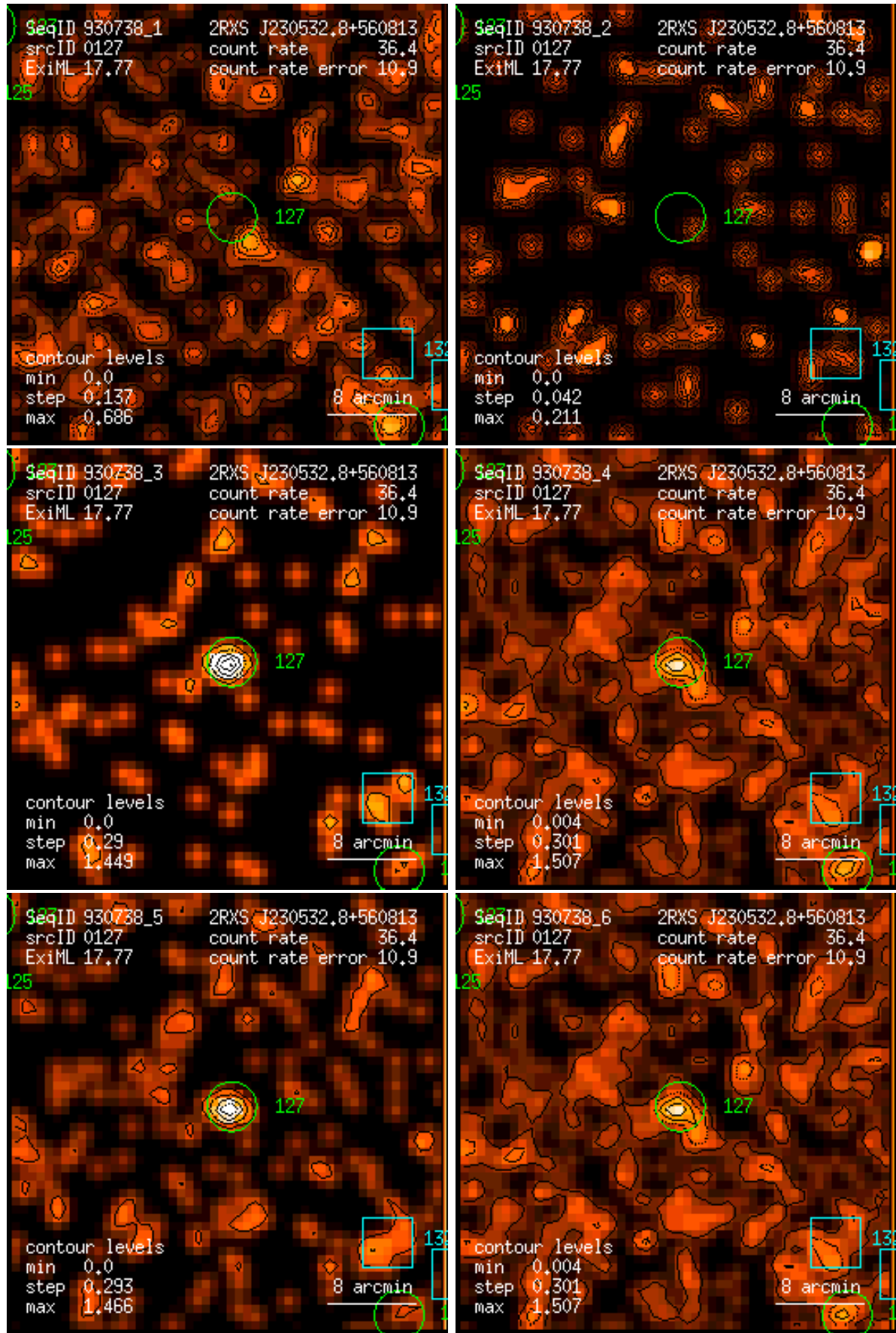
Figure 127: RASS 930738: detection 0127: band rate images, Gaussian filter: (1) PSPC channels 11 – 41, (2) 52 – 90, (3) 91 – 201, (4) 11 – 235, (5) 52 – 201, (6) 11 – 201. Broad band rates in counts/ks. Band rate contour levels in counts/ks/arcmin 2 .
