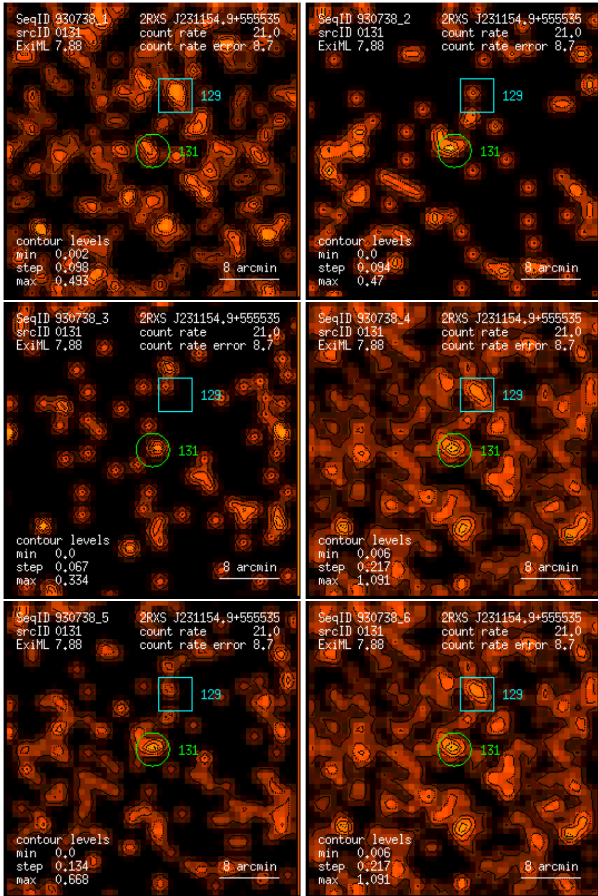
Figure 131: RASS 930738: detection 0131: band rate images, Gaussian filter: (1) PSPC channels 11 – 41, (2) 52 – 90, (3) 91 – 201, (4) 11 – 235, (5) 52 – 201, (6) 11 – 201. Broad band rates in counts/ks. Band rate contour levels in counts/ks/arcmin 2 .
