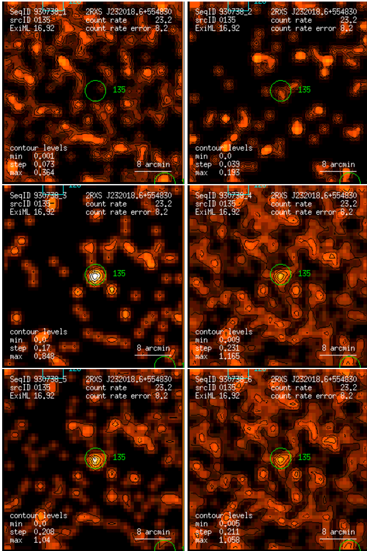
Figure 135: RASS 930738: detection 0135: band rate images, Gaussian filter: (1) PSPC channels 11 – 41, (2) 52 – 90, (3) 91 – 201, (4) 11 – 235, (5) 52 – 201, (6) 11 – 201. Broad band rates in counts/ks. Band rate contour levels in counts/ks/arcmin 2 .
