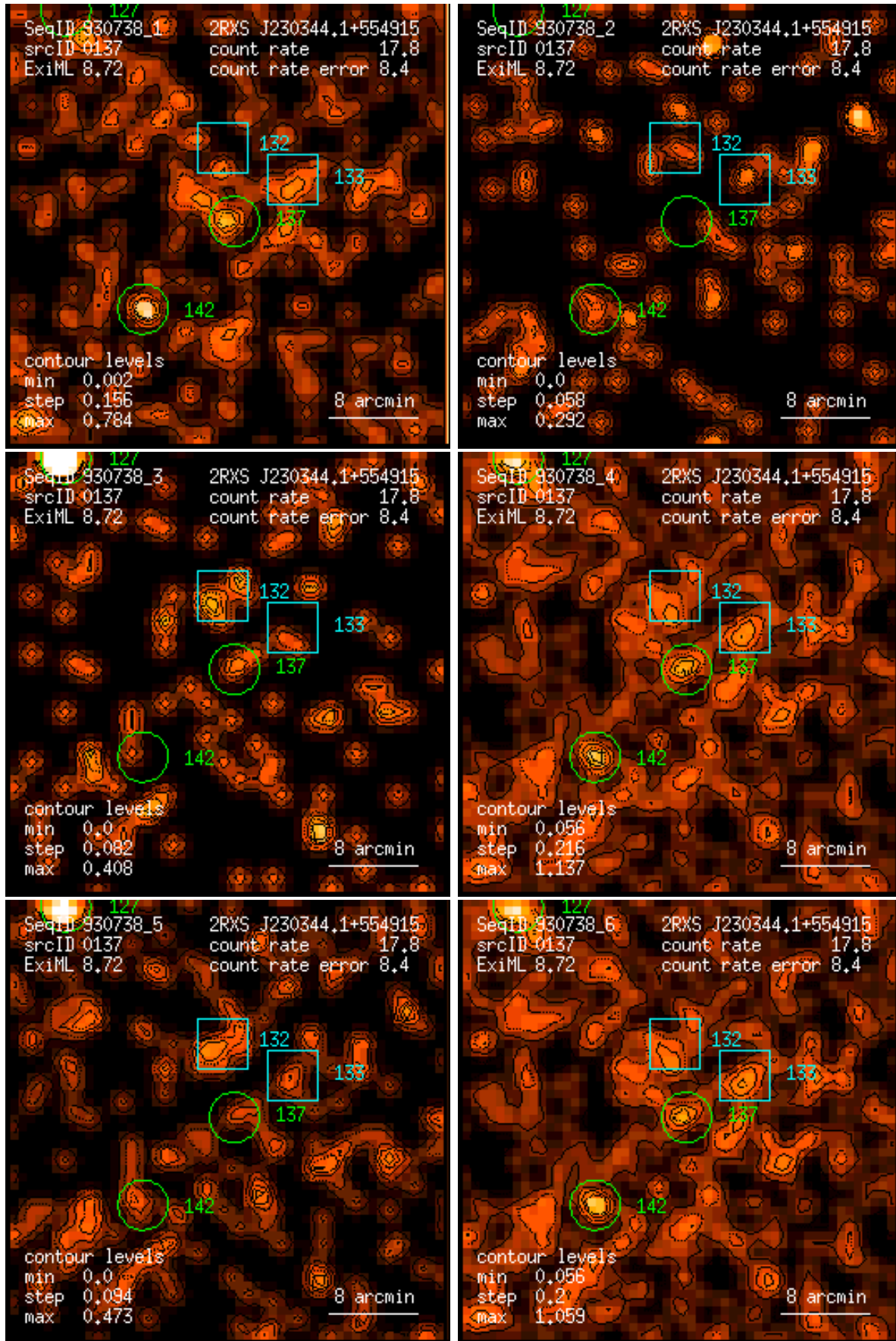
Figure 137: RASS 930738: detection 0137: band rate images, Gaussian filter: (1) PSPC channels 11 – 41, (2) 52 – 90, (3) 91 – 201, (4) 11 – 235, (5) 52 – 201, (6) 11 – 201. Broad band rates in counts/ks. Band rate contour levels in counts/ks/arcmin 2 .
