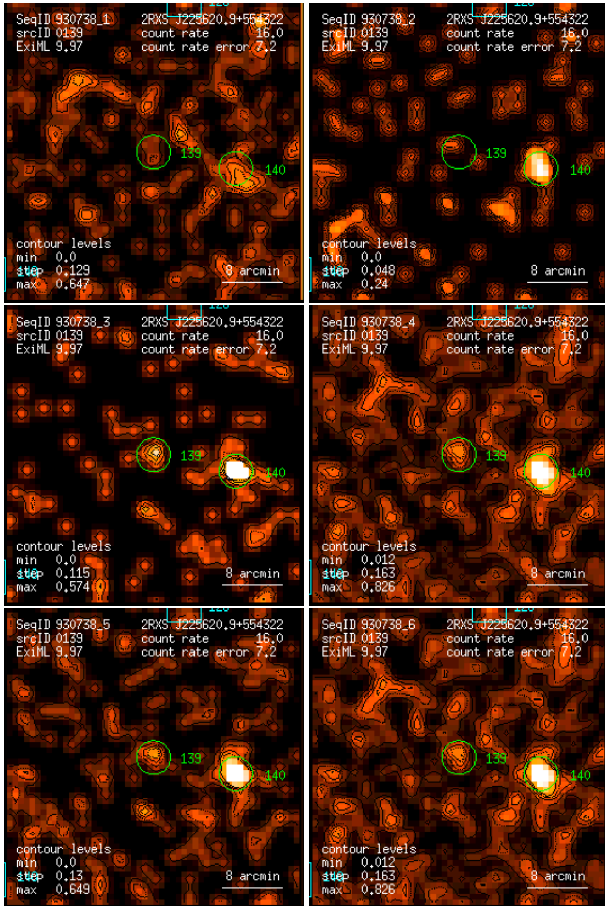
Figure 139: RASS 930738: detection 0139: band rate images, Gaussian filter: (1) PSPC channels 11 – 41, (2) 52 – 90, (3) 91 – 201, (4) 11 – 235, (5) 52 – 201, (6) 11 – 201. Broad band rates in counts/ks. Band rate contour levels in counts/ks/arcmin 2 .
