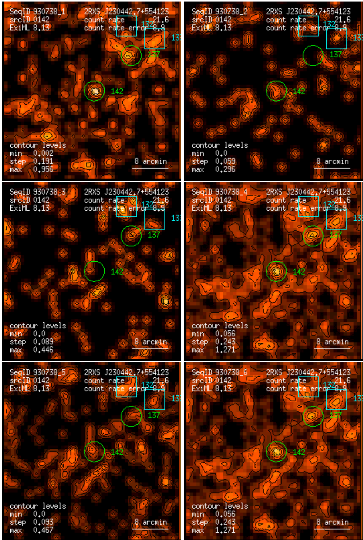
Figure 142: RASS 930738: detection 0142: band rate images, Gaussian filter: (1) PSPC channels 11 – 41, (2) 52 – 90, (3) 91 – 201, (4) 11 – 235, (5) 52 – 201, (6) 11 – 201. Broad band rates in counts/ks. Band rate contour levels in counts/ks/arcmin 2 .
