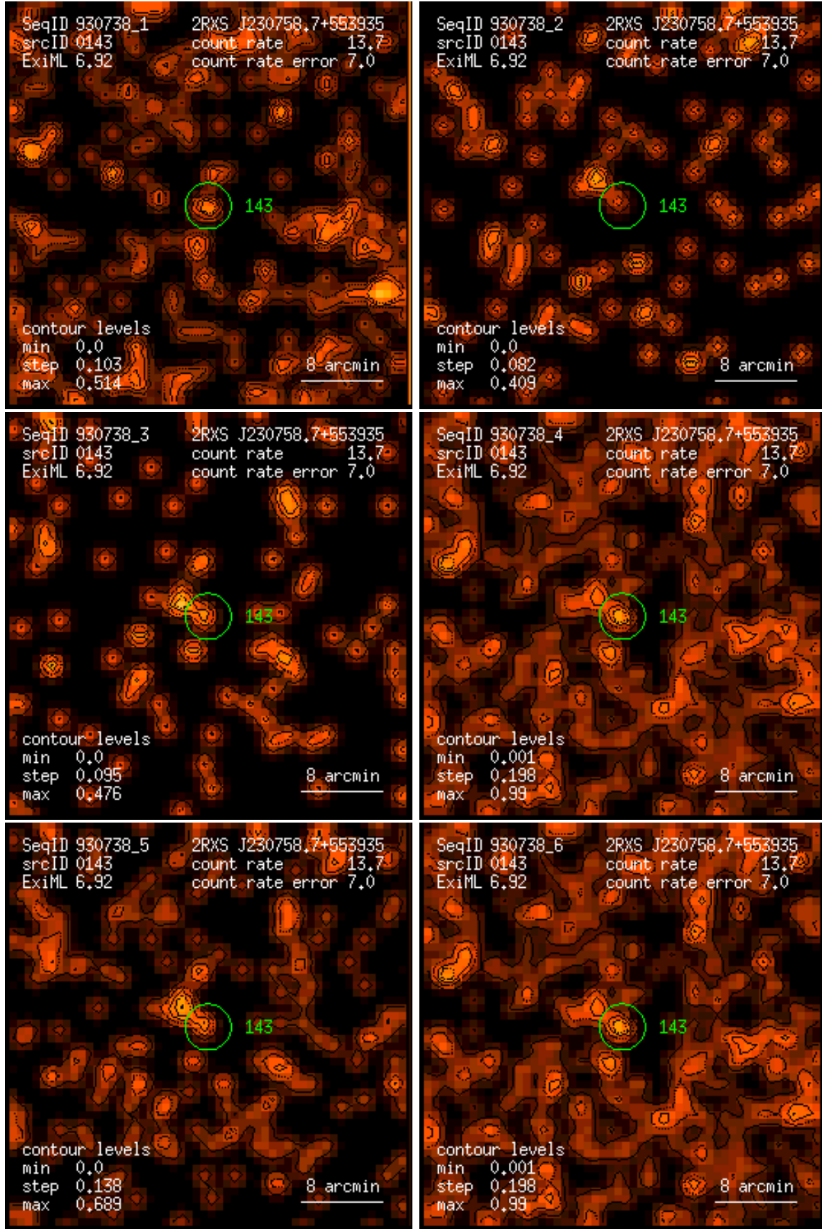
Figure 143: RASS 930738: detection 0143: band rate images, Gaussian filter: (1) PSPC channels 11 – 41, (2) 52 – 90, (3) 91 – 201, (4) 11 – 235, (5) 52 – 201, (6) 11 – 201. Broad band rates in counts/ks. Band rate contour levels in counts/ks/arcmin 2 .
