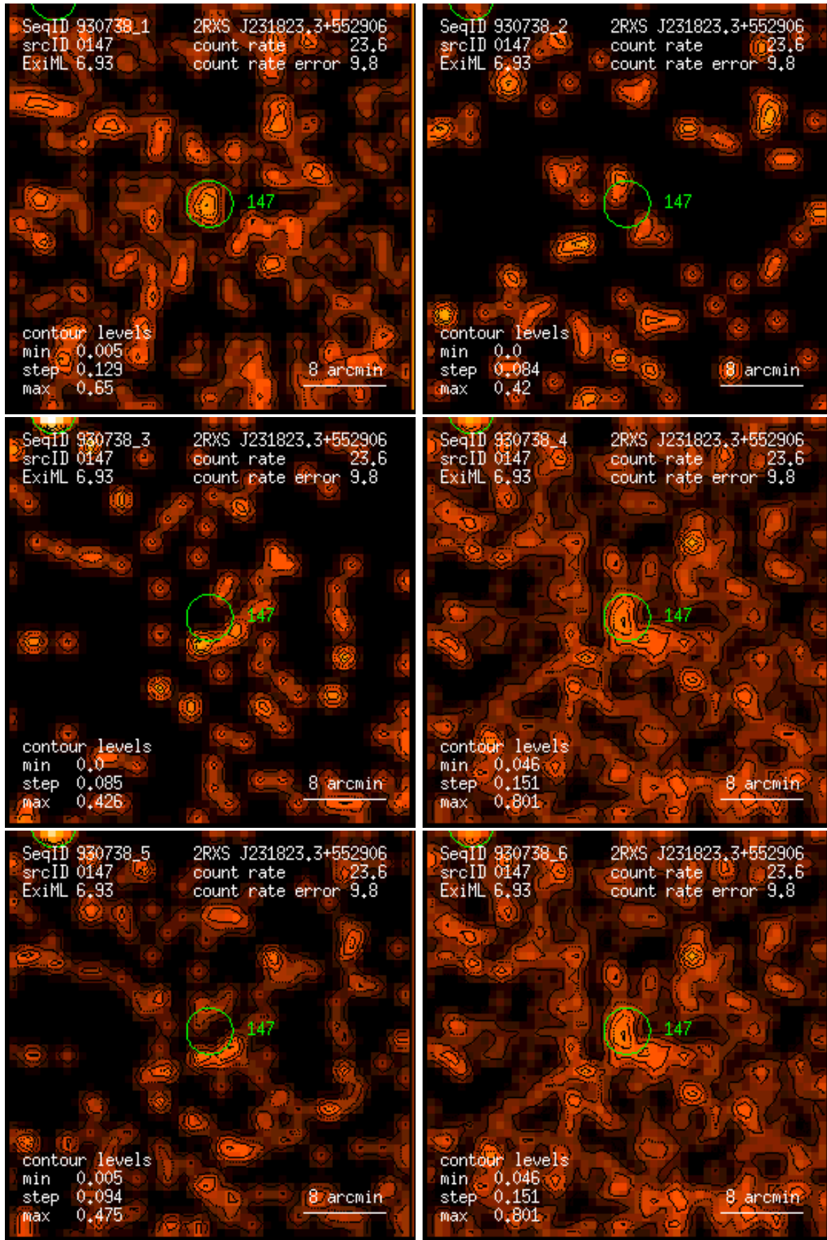
Figure 147: RASS 930738: detection 0147: band rate images, Gaussian filter: (1) PSPC channels 11 – 41, (2) 52 – 90, (3) 91 – 201, (4) 11 – 235, (5) 52 – 201, (6) 11 – 201. Broad band rates in counts/ks. Band rate contour levels in counts/ks/arcmin 2 .
