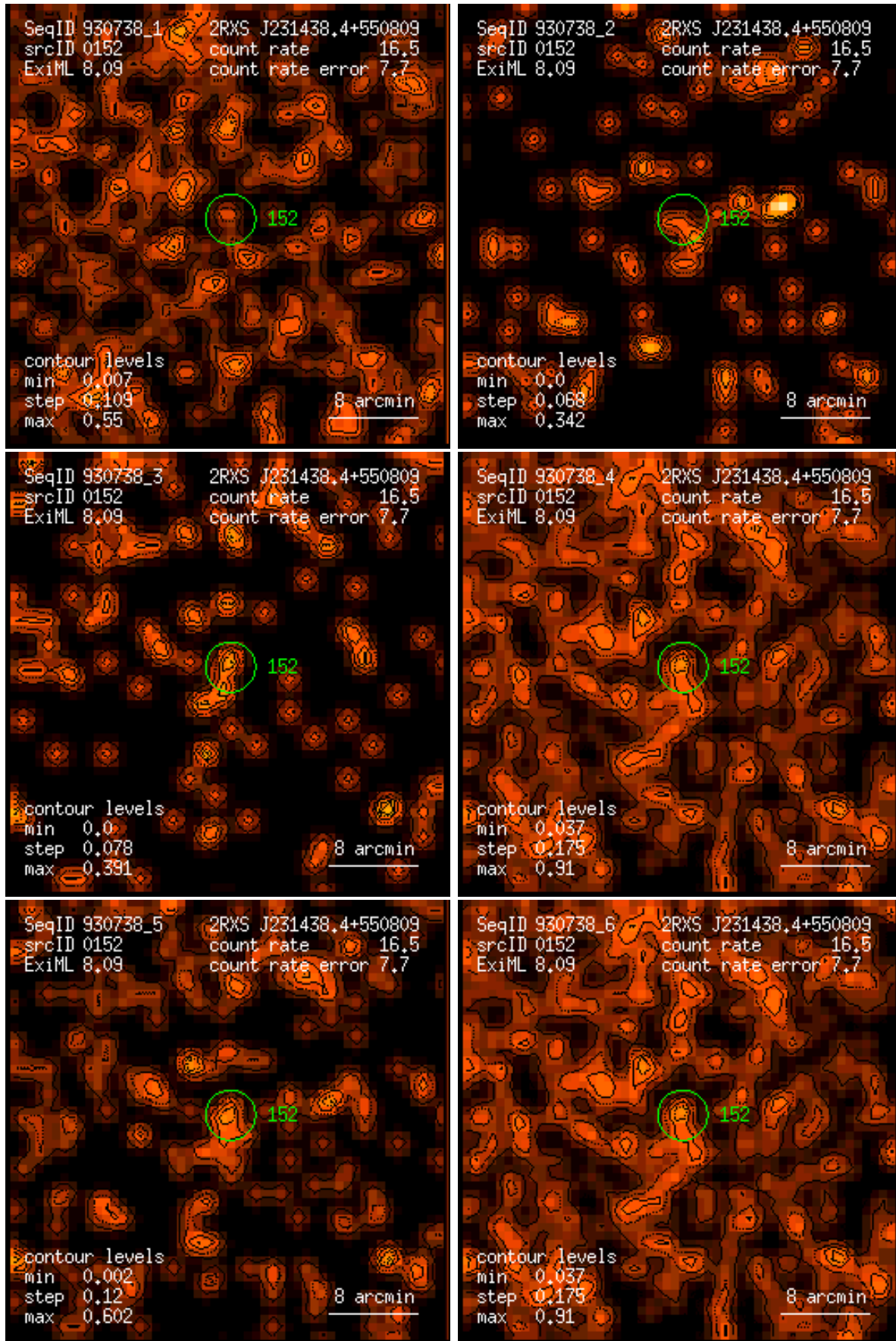
Figure 152: RASS 930738: detection 0152: band rate images, Gaussian filter: (1) PSPC channels 11 – 41, (2) 52 – 90, (3) 91 – 201, (4) 11 – 235, (5) 52 – 201, (6) 11 – 201. Broad band rates in counts/ks. Band rate contour levels in counts/ks/arcmin 2 .
