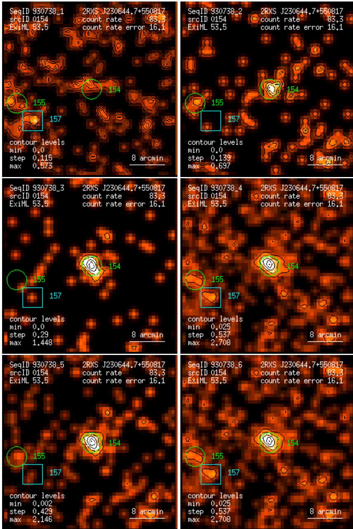
Figure 154: RASS 930738: detection 0154: band rate images, Gaussian filter: (1) PSPC channels 11 – 41, (2) 52 – 90, (3) 91 – 201, (4) 11 – 235, (5) 52 – 201, (6) 11 – 201. Broad band rates in counts/ks. Band rate contour levels in counts/ks/arcmin 2 .
