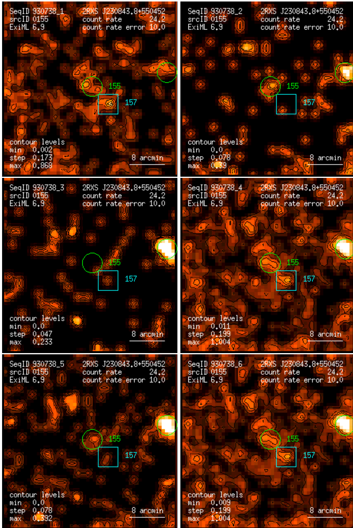
Figure 155: RASS 930738: detection 0155: band rate images, Gaussian filter: (1) PSPC channels 11 – 41, (2) 52 – 90, (3) 91 – 201, (4) 11 – 235, (5) 52 – 201, (6) 11 – 201. Broad band rates in counts/ks. Band rate contour levels in counts/ks/arcmin 2 .
