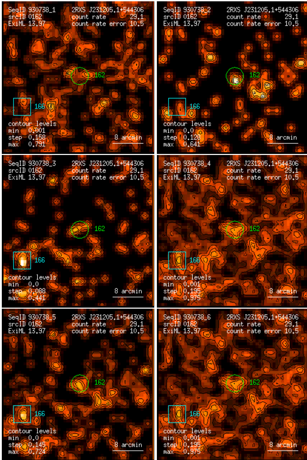
Figure 162: RASS 930738: detection 0162: band rate images, Gaussian filter: (1) PSPC channels 11 – 41, (2) 52 – 90, (3) 91 – 201, (4) 11 – 235, (5) 52 – 201, (6) 11 – 201. Broad band rates in counts/ks. Band rate contour levels in counts/ks/arcmin 2 .
