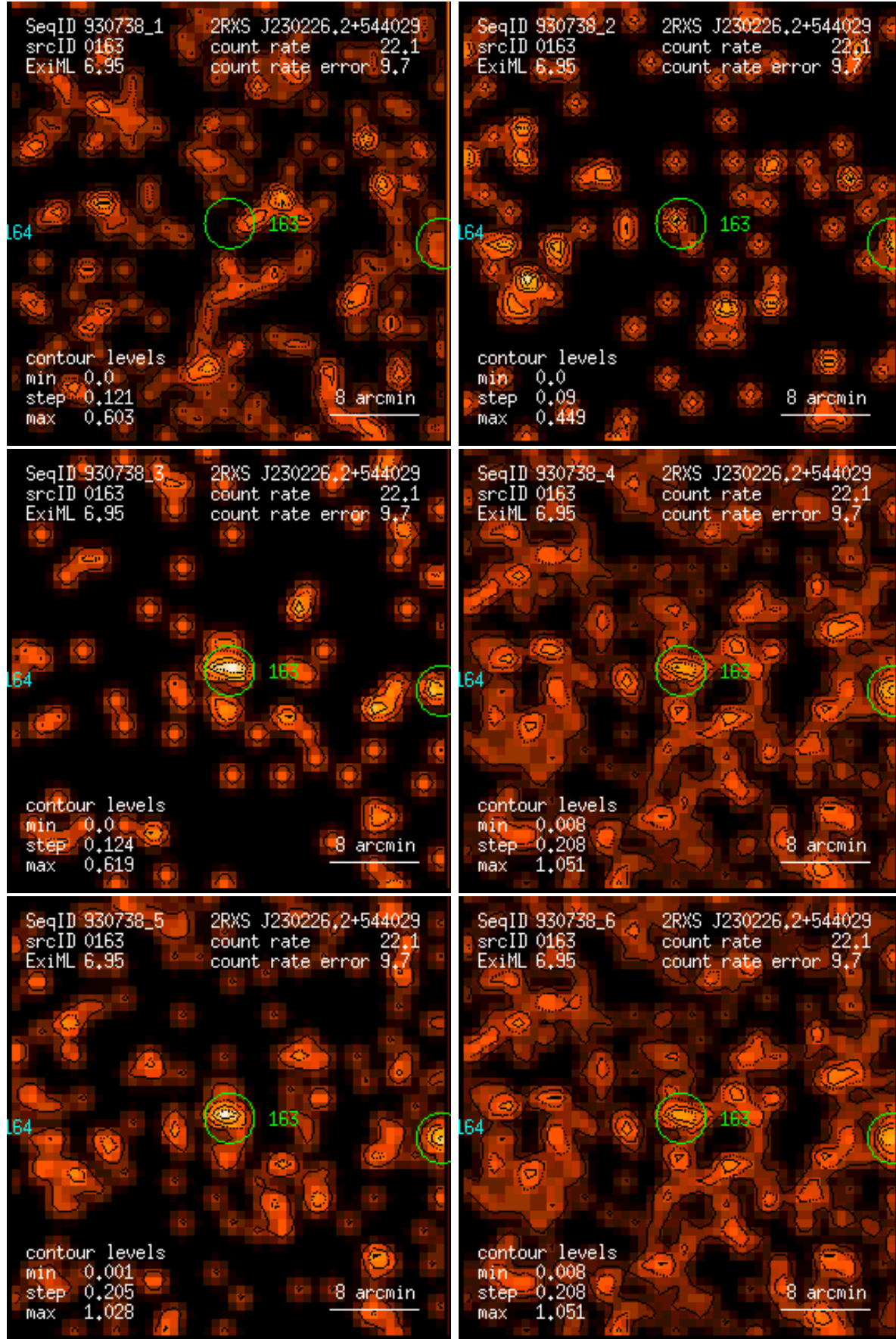
Figure 163: RASS 930738: detection 0163: band rate images, Gaussian filter: (1) PSPC channels 11 – 41, (2) 52 – 90, (3) 91 – 201, (4) 11 – 235, (5) 52 – 201, (6) 11 – 201. Broad band rates in counts/ks. Band rate contour levels in counts/ks/arcmin 2 .
