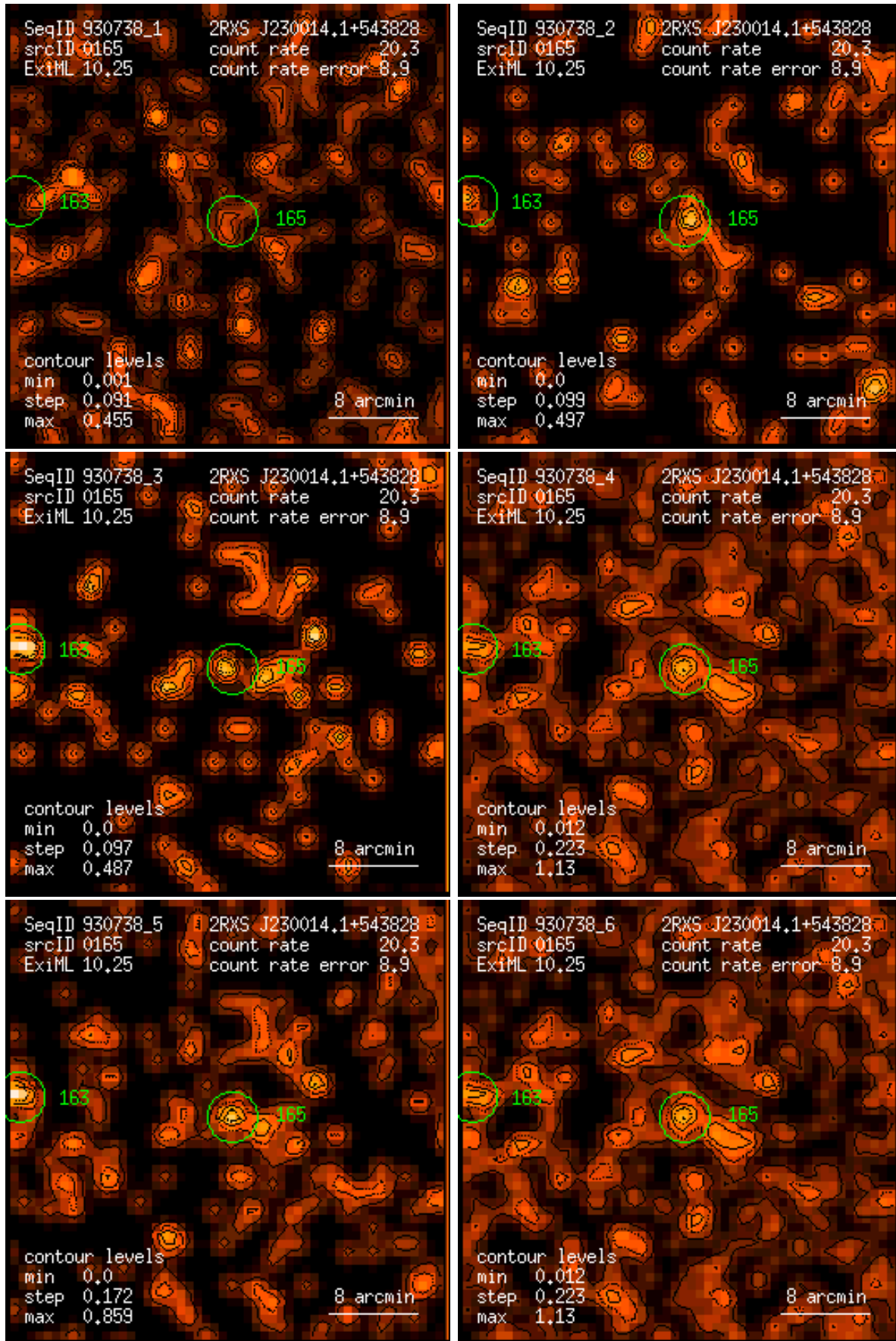
Figure 165: RASS 930738: detection 0165: band rate images, Gaussian filter: (1) PSPC channels 11 – 41, (2) 52 – 90, (3) 91 – 201, (4) 11 – 235, (5) 52 – 201, (6) 11 – 201. Broad band rates in counts/ks. Band rate contour levels in counts/ks/arcmin 2 .
