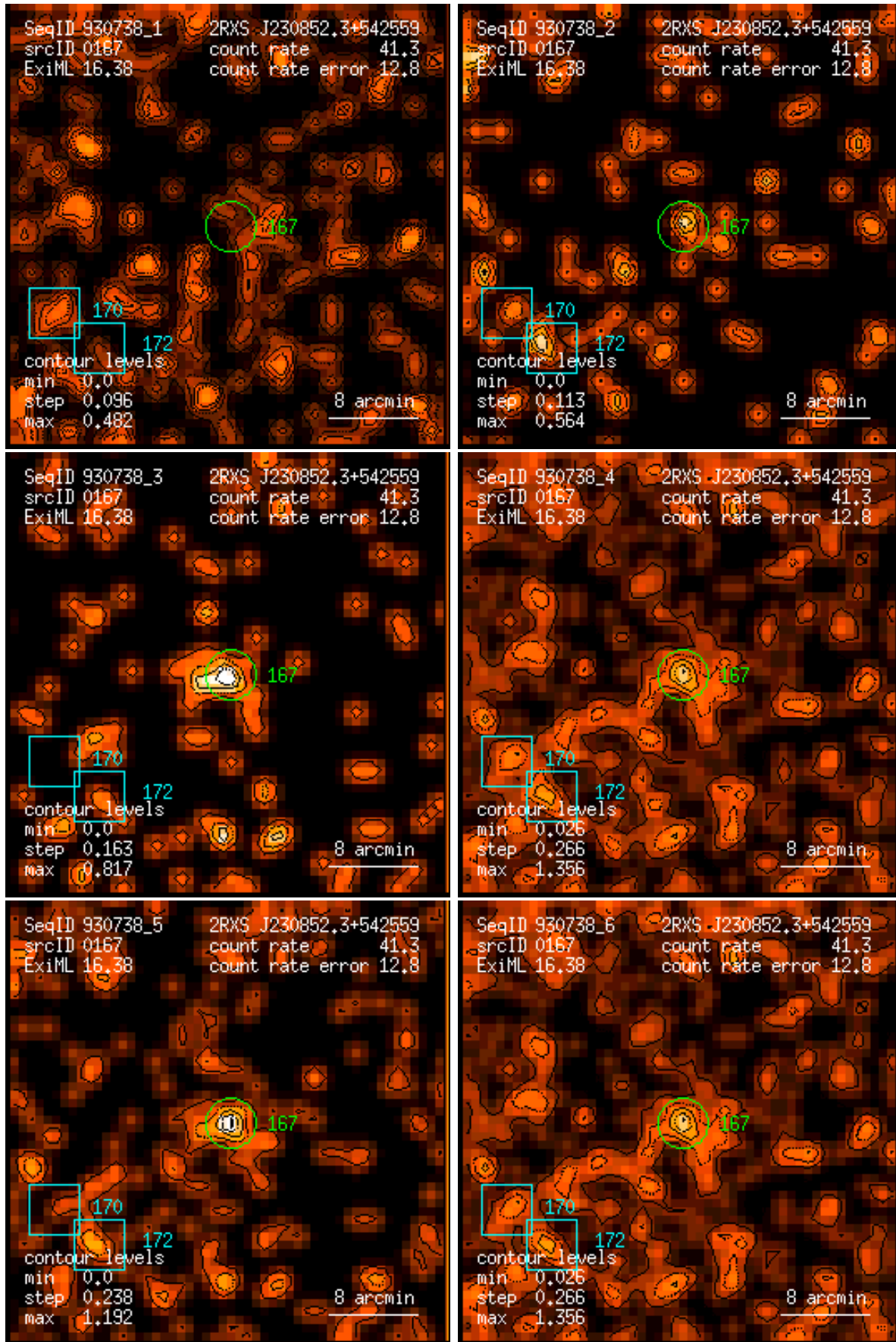
Figure 167: RASS 930738: detection 0167: band rate images, Gaussian filter: (1) PSPC channels 11 – 41, (2) 52 – 90, (3) 91 – 201, (4) 11 – 235, (5) 52 – 201, (6) 11 – 201. Broad band rates in counts/ks. Band rate contour levels in counts/ks/arcmin 2 .
