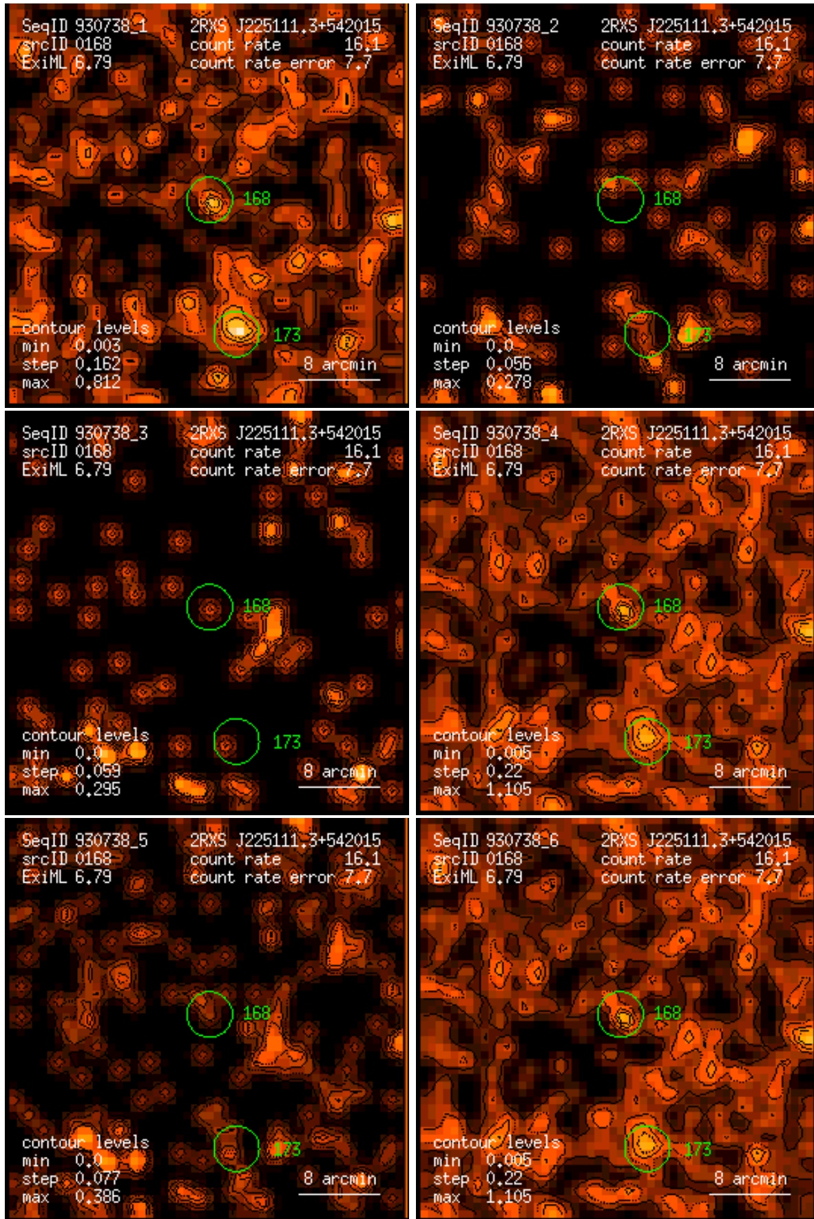
Figure 168: RASS 930738: detection 0168: band rate images, Gaussian filter: (1) PSPC channels 11 – 41, (2) 52 – 90, (3) 91 – 201, (4) 11 – 235, (5) 52 – 201, (6) 11 – 201. Broad band rates in counts/ks. Band rate contour levels in counts/ks/arcmin 2 .
