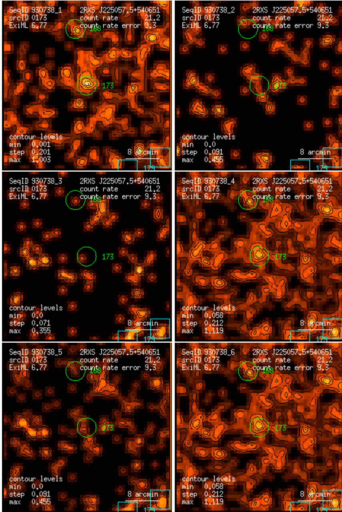
Figure 173: RASS 930738: detection 0173: band rate images, Gaussian filter: (1) PSPC channels 11 – 41, (2) 52 – 90, (3) 91 – 201, (4) 11 – 235, (5) 52 – 201, (6) 11 – 201. Broad band rates in counts/ks. Band rate contour levels in counts/ks/arcmin 2 .
