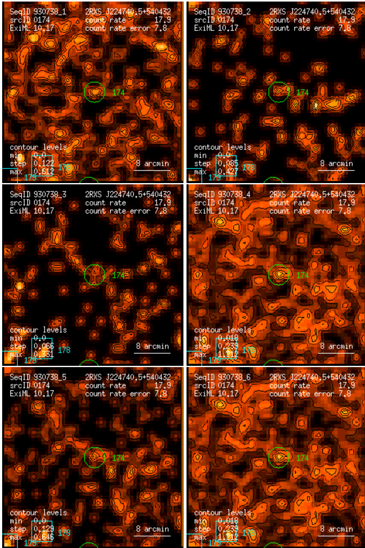
Figure 174: RASS 930738: detection 0174: band rate images, Gaussian filter: (1) PSPC channels 11 – 41, (2) 52 – 90, (3) 91 – 201, (4) 11 – 235, (5) 52 – 201, (6) 11 – 201. Broad band rates in counts/ks. Band rate contour levels in counts/ks/arcmin 2 .
