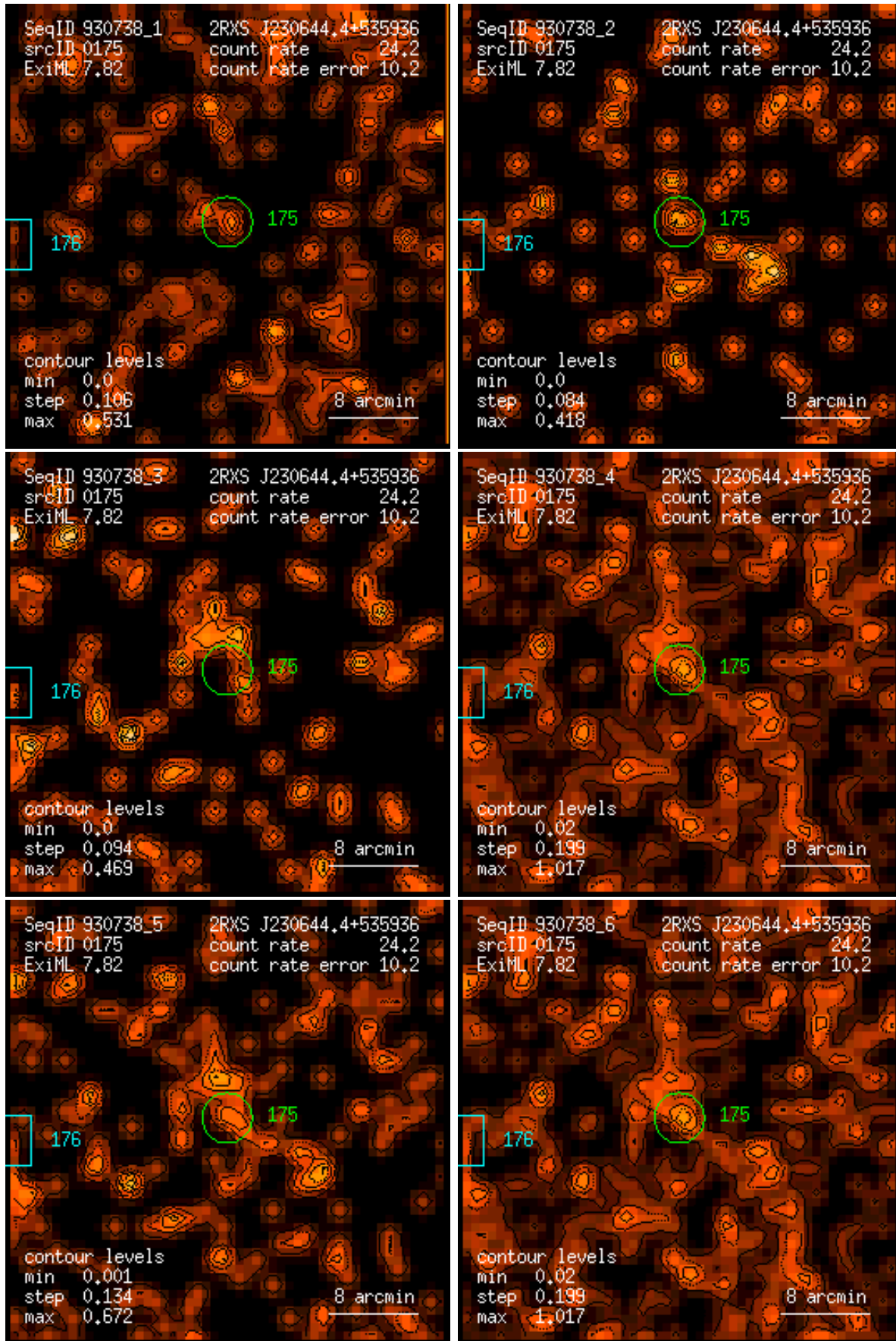
Figure 175: RASS 930738: detection 0175: band rate images, Gaussian filter: (1) PSPC channels 11 – 41, (2) 52 – 90, (3) 91 – 201, (4) 11 – 235, (5) 52 – 201, (6) 11 – 201. Broad band rates in counts/ks. Band rate contour levels in counts/ks/arcmin 2 .
