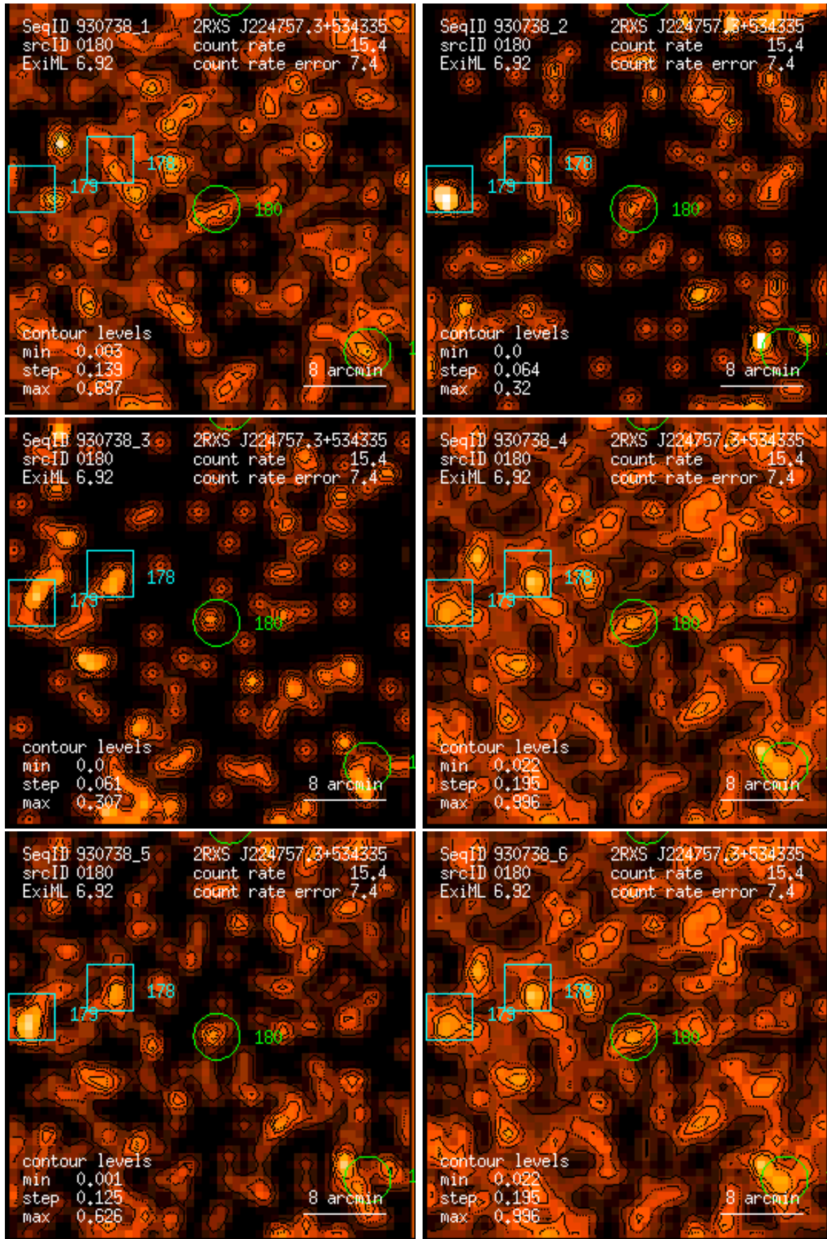
Figure 180: RASS 930738: detection 0180: band rate images, Gaussian filter: (1) PSPC channels 11 – 41, (2) 52 – 90, (3) 91 – 201, (4) 11 – 235, (5) 52 – 201, (6) 11 – 201. Broad band rates in counts/ks. Band rate contour levels in counts/ks/arcmin 2 .
