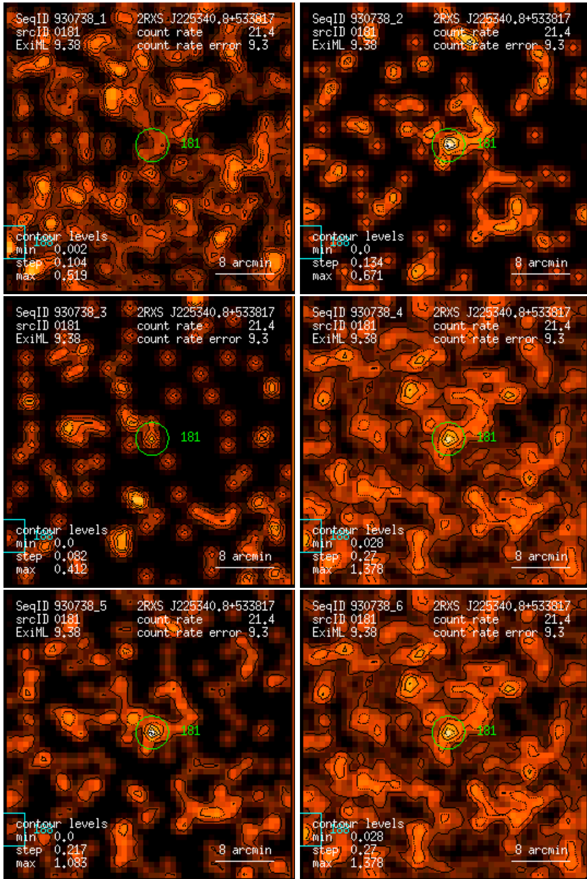
Figure 181: RASS 930738: detection 0181: band rate images, Gaussian filter: (1) PSPC channels 11 – 41, (2) 52 – 90, (3) 91 – 201, (4) 11 – 235, (5) 52 – 201, (6) 11 – 201. Broad band rates in counts/ks. Band rate contour levels in counts/ks/arcmin 2 .
