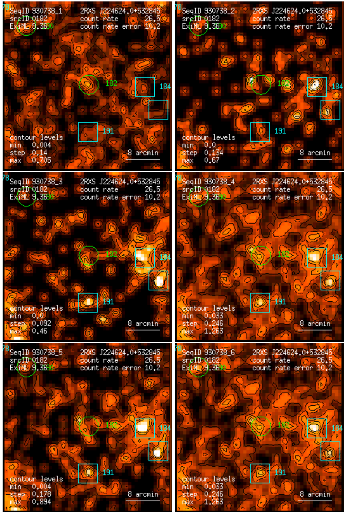
Figure 182: RASS 930738: detection 0182: band rate images, Gaussian filter: (1) PSPC channels 11 – 41, (2) 52 – 90, (3) 91 – 201, (4) 11 – 235, (5) 52 – 201, (6) 11 – 201. Broad band rates in counts/ks. Band rate contour levels in counts/ks/arcmin 2 .
