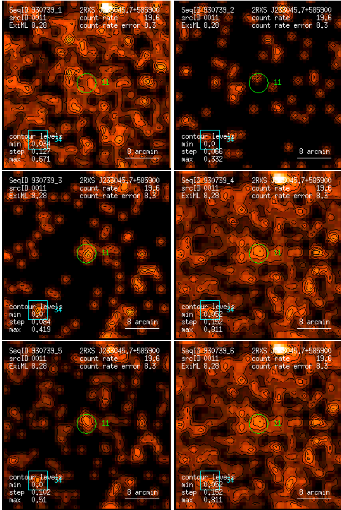
Figure 11: RASS 930739: detection 0011: band rate images, Gaussian filter: (1) PSPC channels 11 – 41, (2) 52 – 90, (3) 91 – 201, (4) 11 – 235, (5) 52 – 201, (6) 11 – 201. Broad band rates in counts/ks. Band rate contour levels in counts/ks/arcmin 2 .
