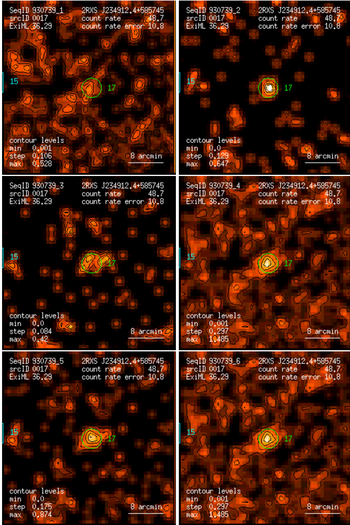
Figure 17: RASS 930739: detection 0017: band rate images, Gaussian filter: (1) PSPC channels 11 – 41, (2) 52 – 90, (3) 91 – 201, (4) 11 – 235, (5) 52 – 201, (6) 11 – 201. Broad band rates in counts/ks. Band rate contour levels in counts/ks/arcmin 2 .
