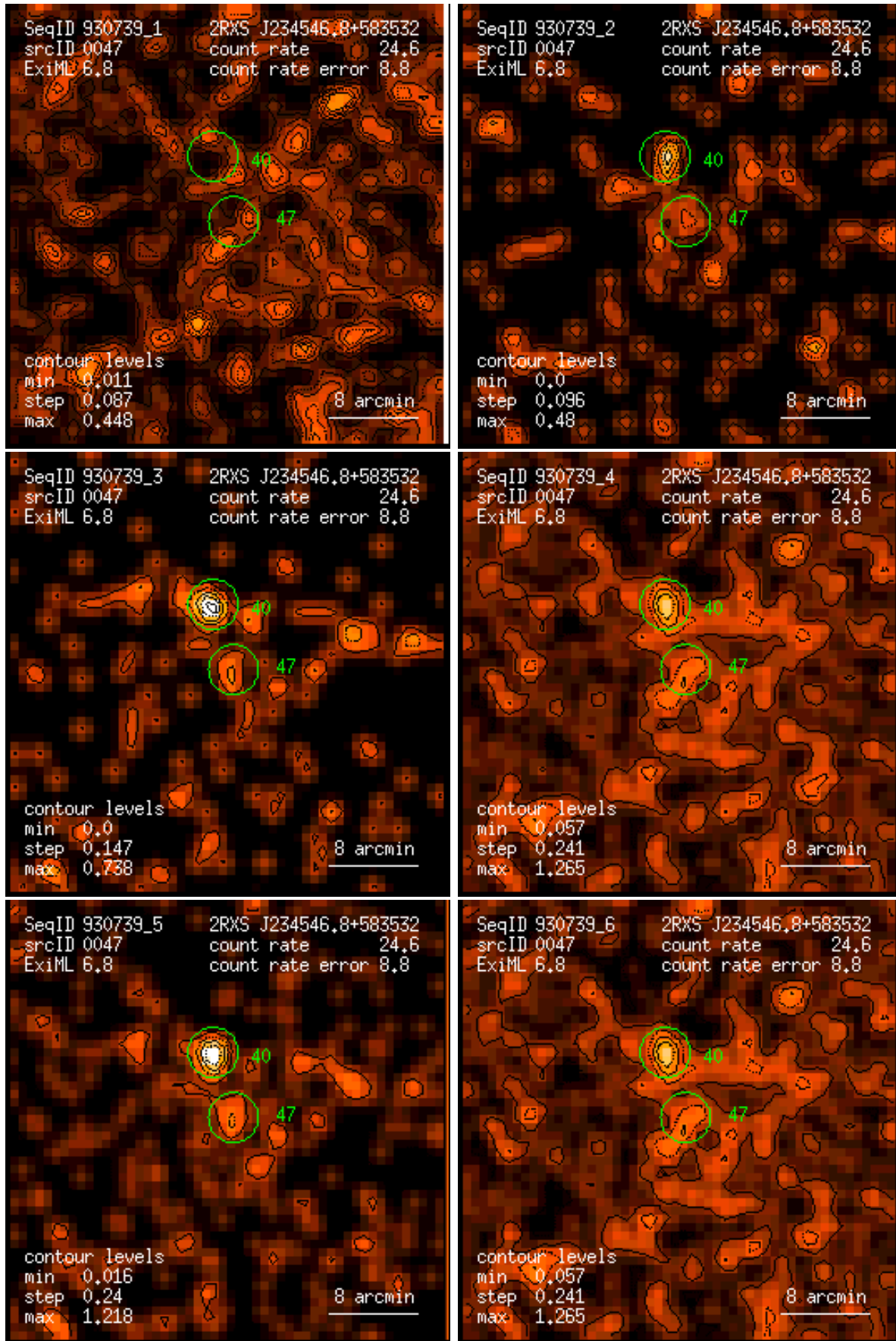
Figure 47: RASS 930739: detection 0047: band rate images, Gaussian filter: (1) PSPC channels 11 – 41, (2) 52 – 90, (3) 91 – 201, (4) 11 – 235, (5) 52 – 201, (6) 11 – 201. Broad band rates in counts/ks. Band rate contour levels in counts/ks/arcmin 2 .
