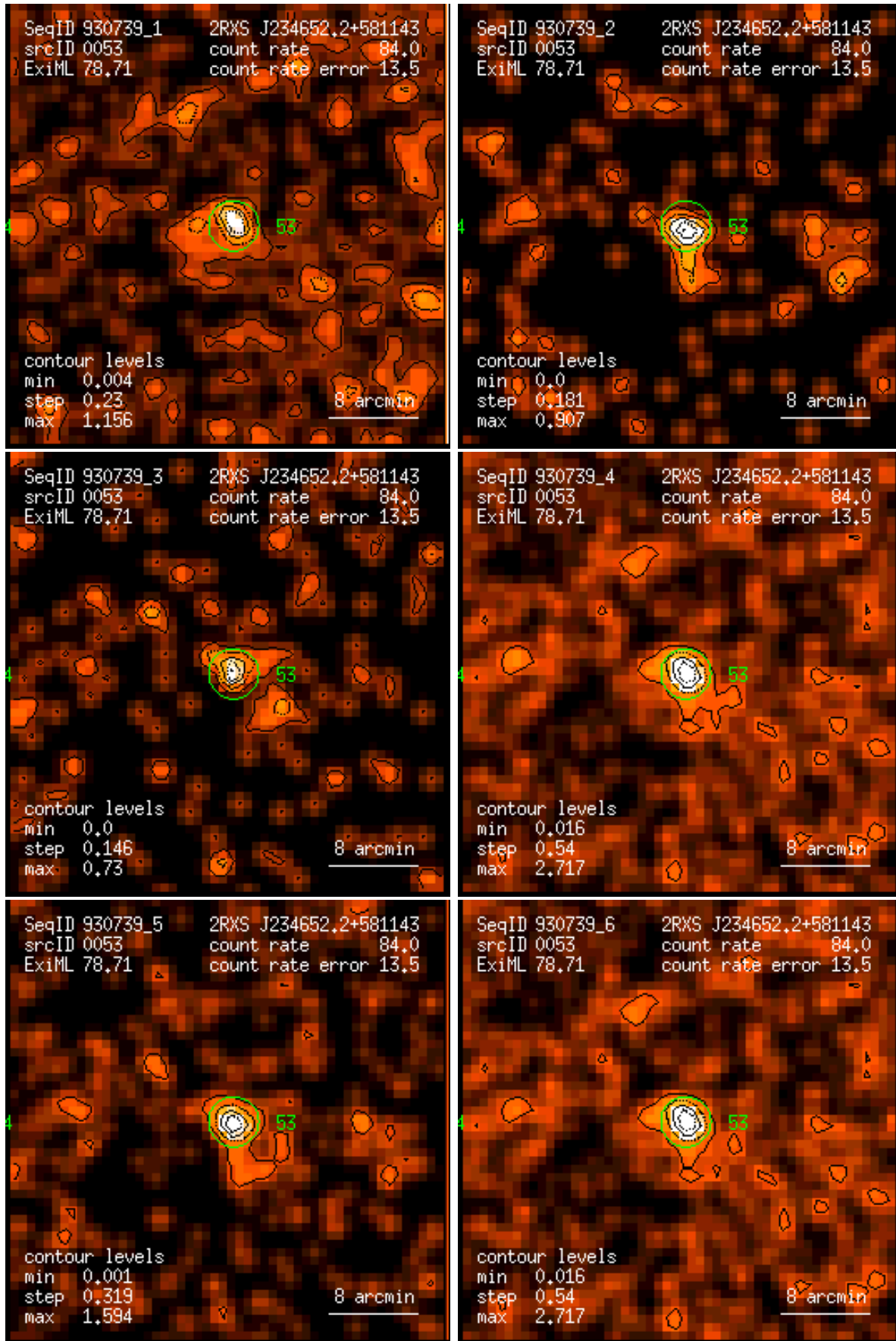
Figure 53: RASS 930739: detection 0053: band rate images, Gaussian filter: (1) PSPC channels 11 – 41, (2) 52 – 90, (3) 91 – 201, (4) 11 – 235, (5) 52 – 201, (6) 11 – 201. Broad band rates in counts/ks. Band rate contour levels in counts/ks/arcmin 2 .
