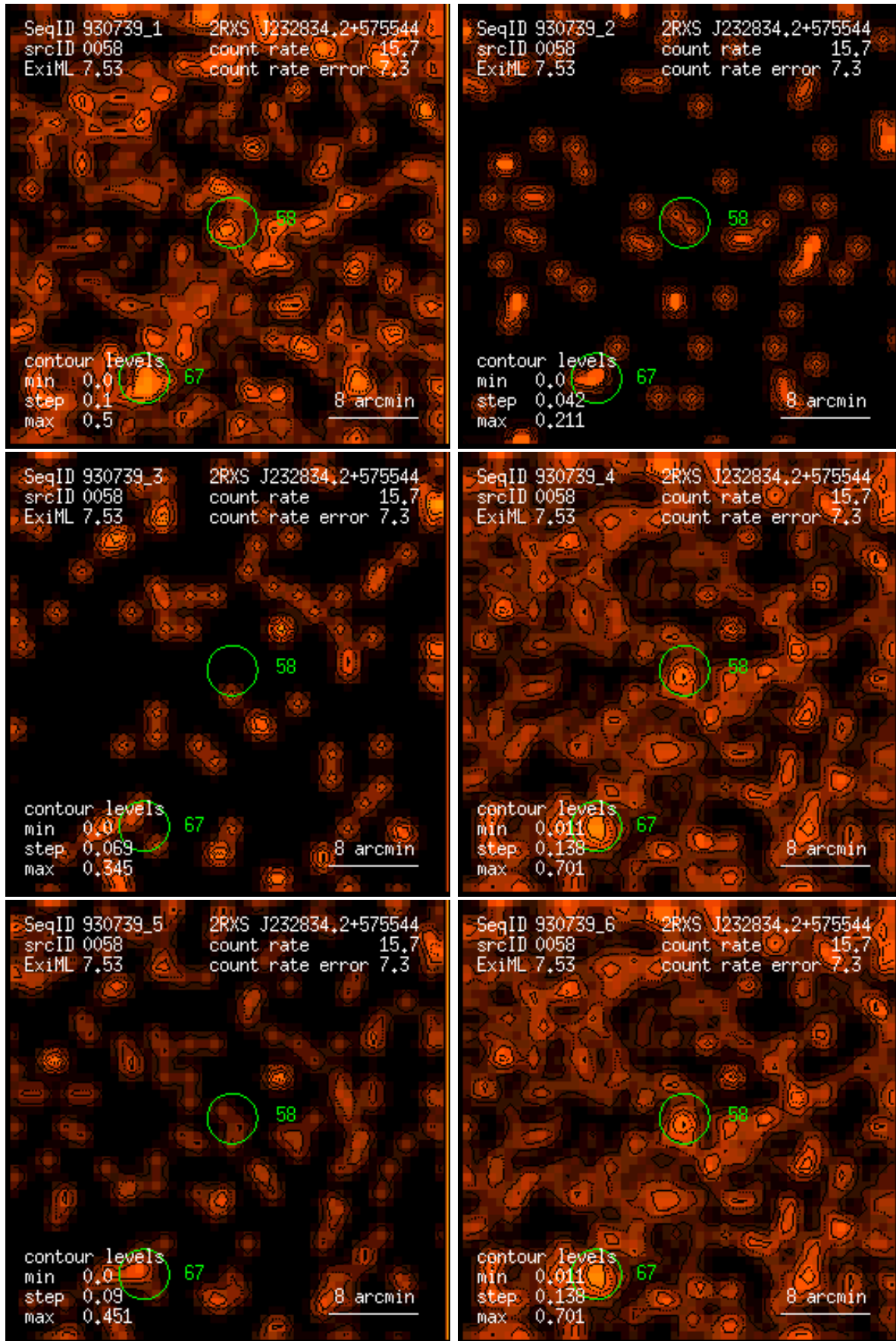
Figure 58: RASS 930739: detection 0058: band rate images, Gaussian filter: (1) PSPC channels 11 – 41, (2) 52 – 90, (3) 91 – 201, (4) 11 – 235, (5) 52 – 201, (6) 11 – 201. Broad band rates in counts/ks. Band rate contour levels in counts/ks/arcmin 2 .
