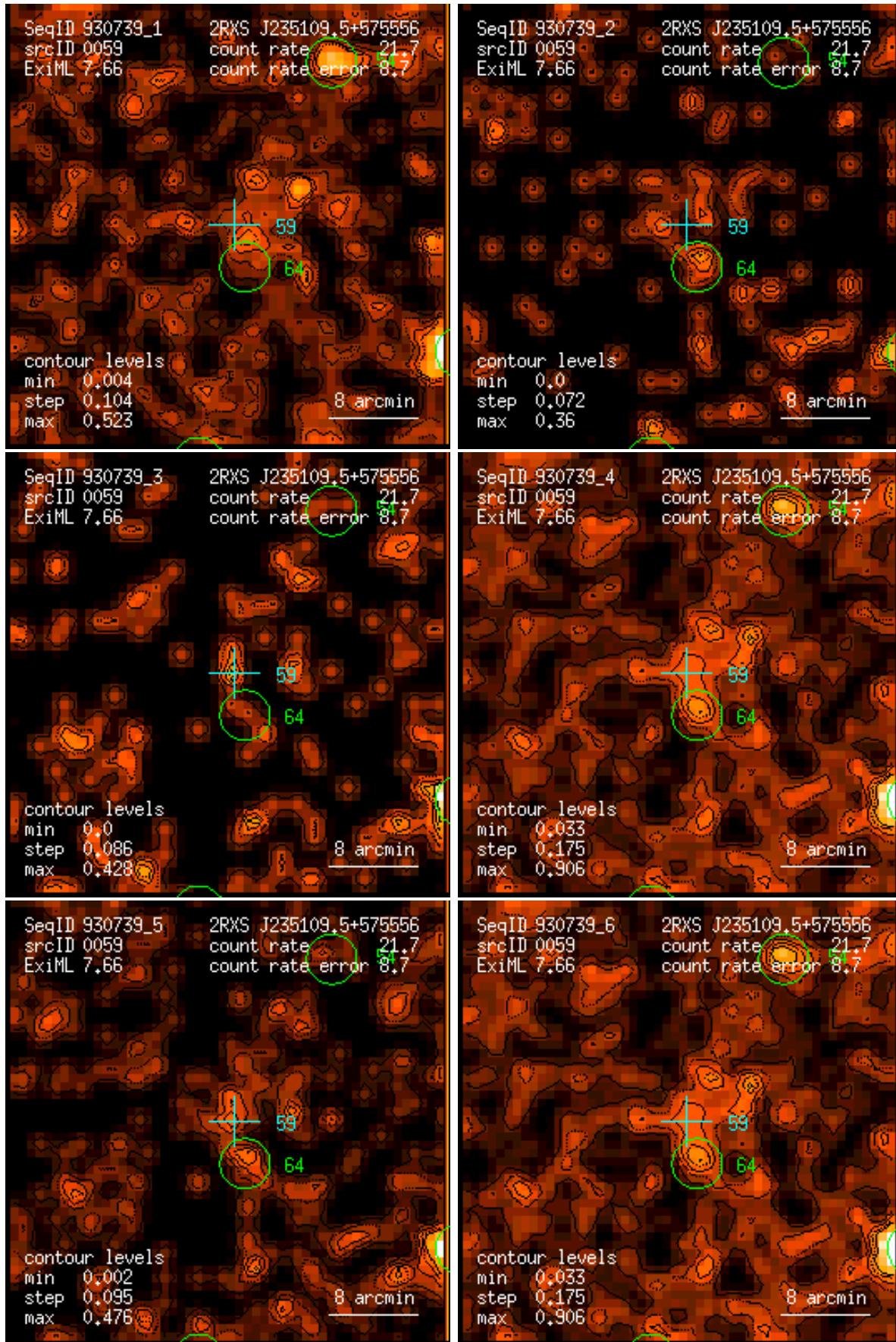
Figure 59: RASS 930739: detection 0059: band rate images, Gaussian filter: (1) PSPC channels 11 – 41, (2) 52 – 90, (3) 91 – 201, (4) 11 – 235, (5) 52 – 201, (6) 11 – 201. Broad band rates in counts/ks. Band rate contour levels in counts/ks/arcmin 2 .
