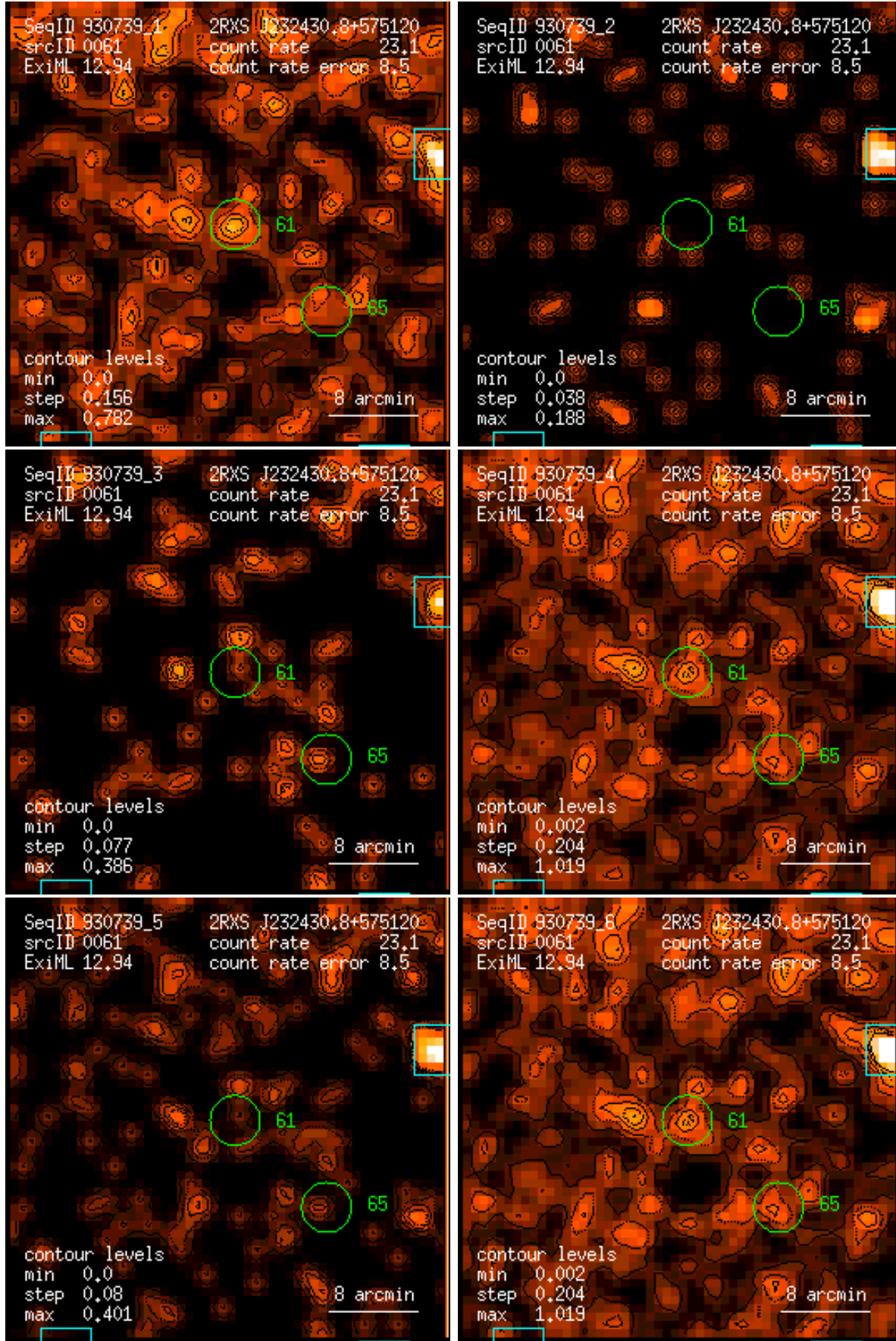
Figure 61: RASS 930739: detection 0061: band rate images, Gaussian filter: (1) PSPC channels 11 – 41, (2) 52 – 90, (3) 91 – 201, (4) 11 – 235, (5) 52 – 201, (6) 11 – 201. Broad band rates in counts/ks. Band rate contour levels in counts/ks/arcmin 2 .
