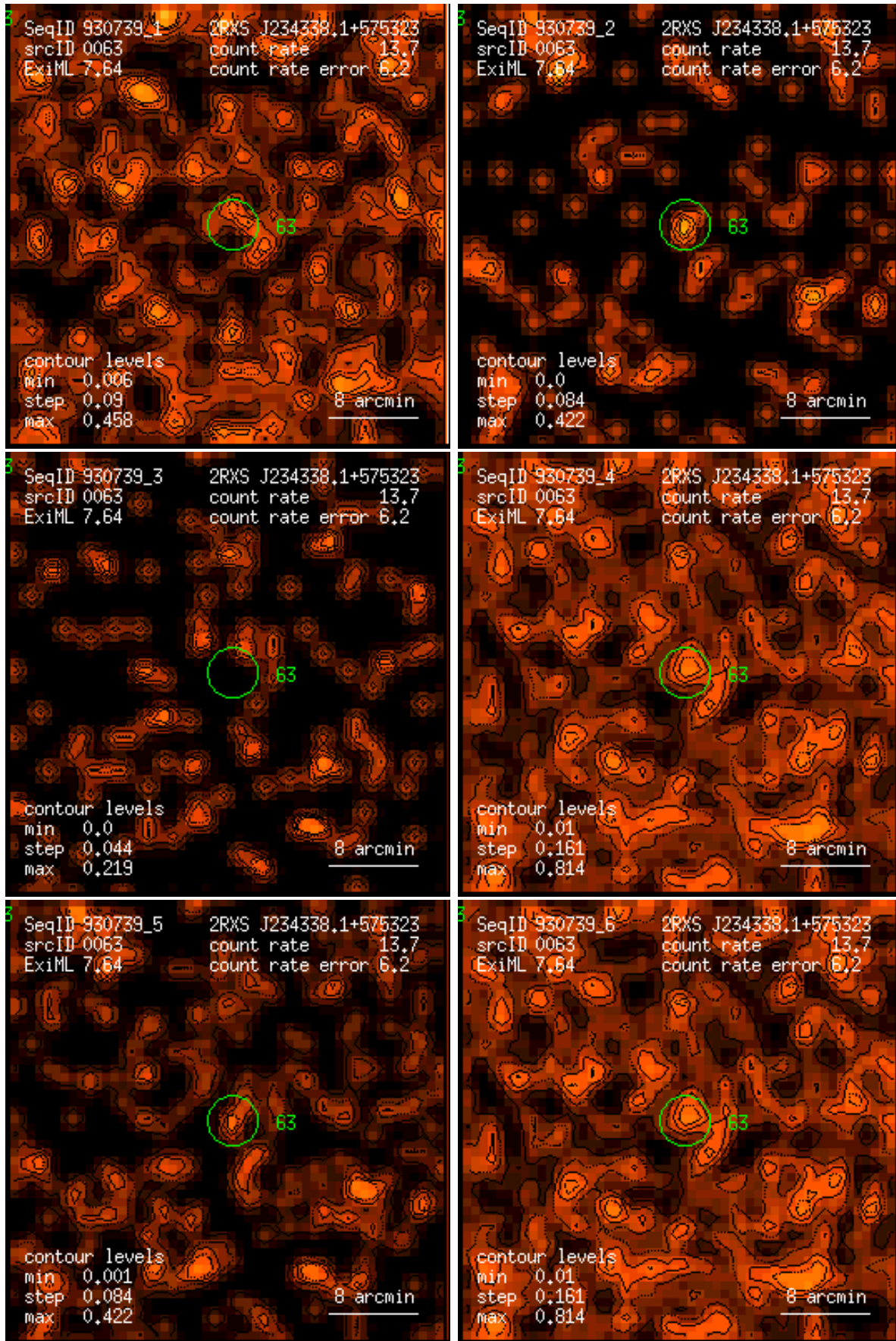
Figure 63: RASS 930739: detection 0063: band rate images, Gaussian filter: (1) PSPC channels 11 – 41, (2) 52 – 90, (3) 91 – 201, (4) 11 – 235, (5) 52 – 201, (6) 11 – 201. Broad band rates in counts/ks. Band rate contour levels in counts/ks/arcmin 2 .
