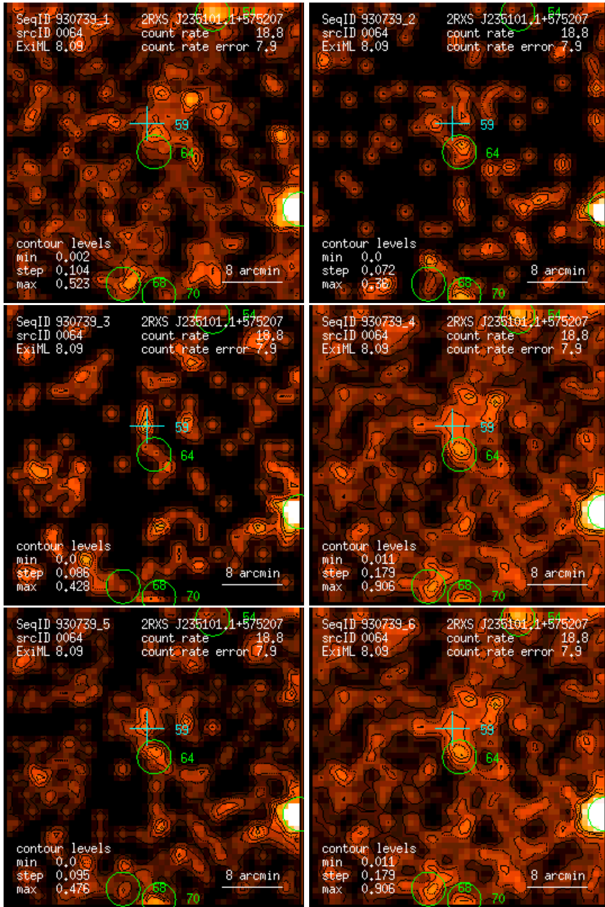
Figure 64: RASS 930739: detection 0064: band rate images, Gaussian filter: (1) PSPC channels 11 – 41, (2) 52 – 90, (3) 91 – 201, (4) 11 – 235, (5) 52 – 201, (6) 11 – 201. Broad band rates in counts/ks. Band rate contour levels in counts/ks/arcmin 2 .
