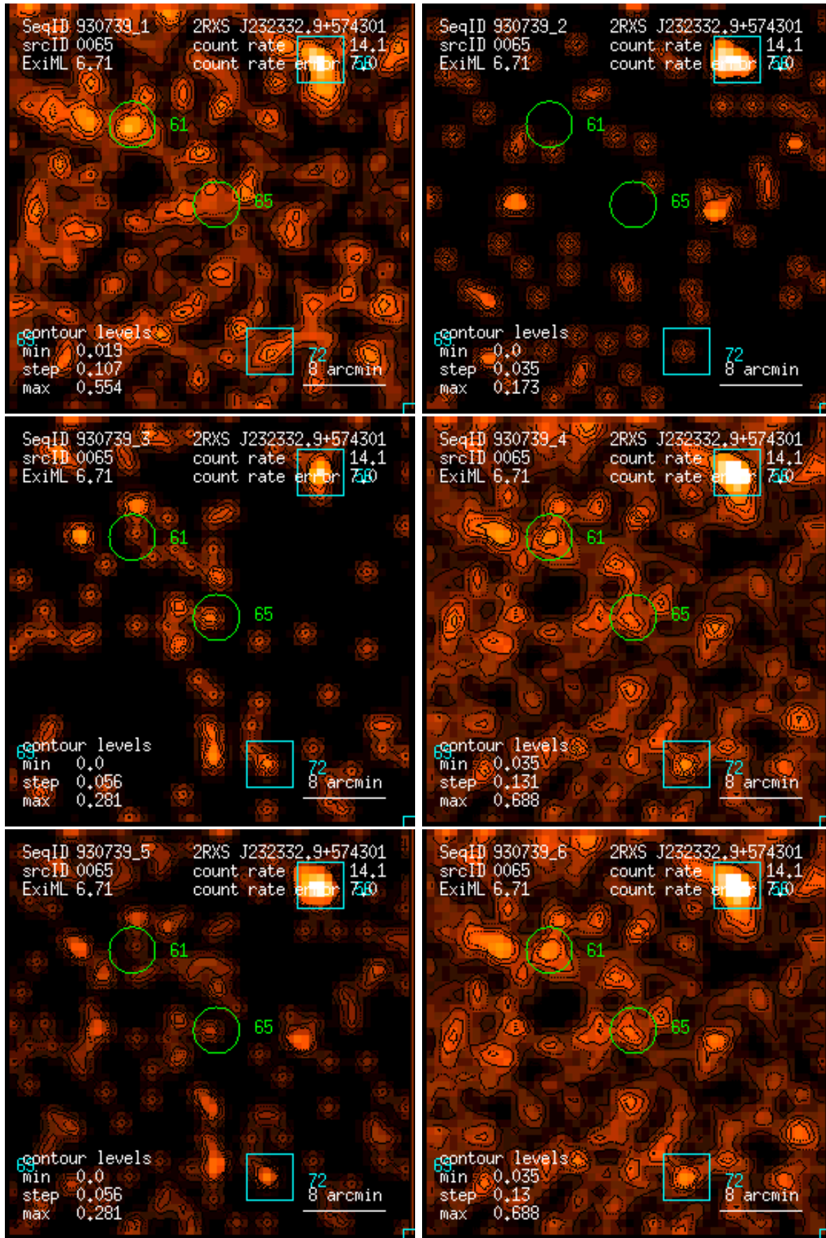
Figure 65: RASS 930739: detection 0065: band rate images, Gaussian filter: (1) PSPC channels 11 – 41, (2) 52 – 90, (3) 91 – 201, (4) 11 – 235, (5) 52 – 201, (6) 11 – 201. Broad band rates in counts/ks. Band rate contour levels in counts/ks/arcmin 2 .
