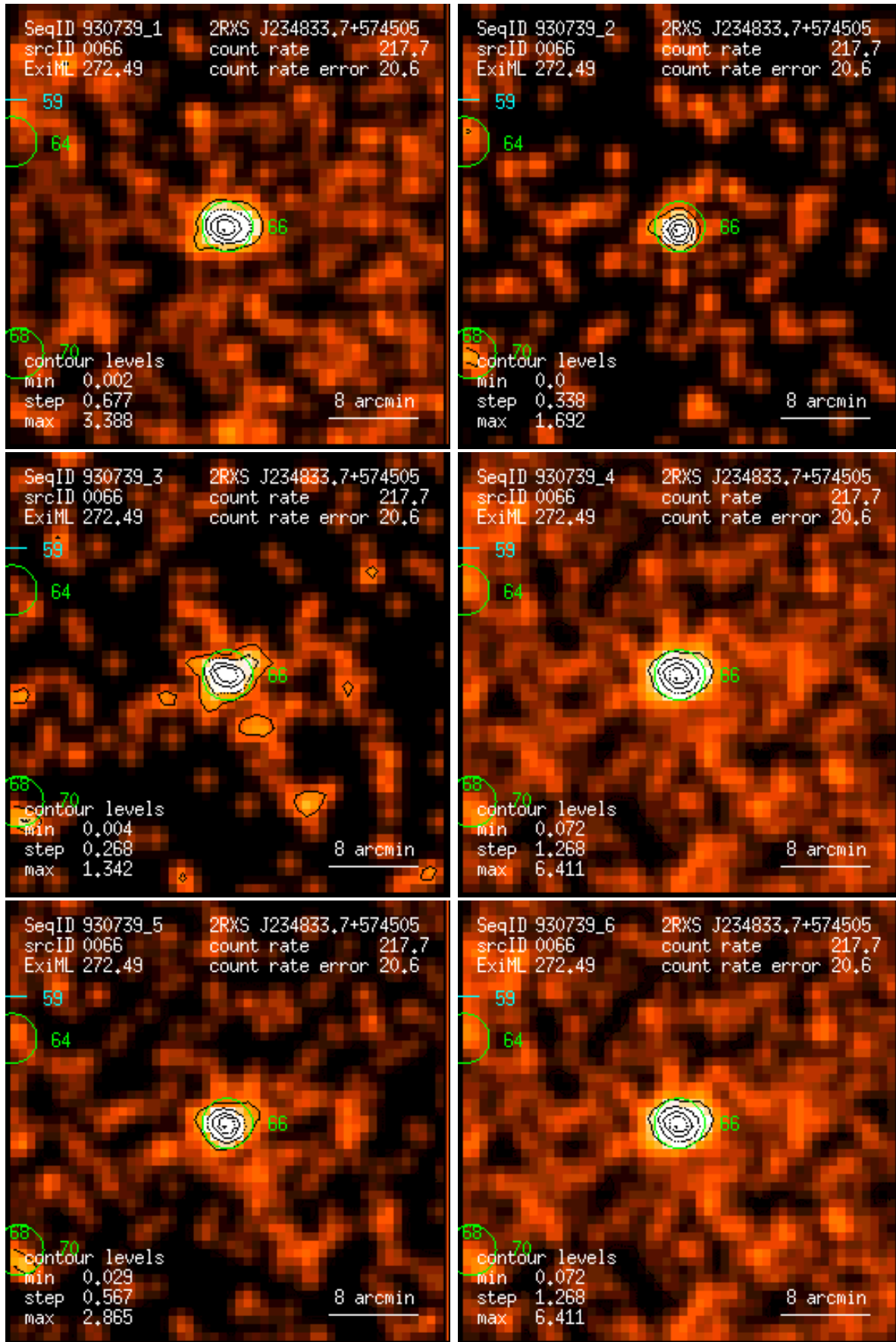
Figure 66: RASS 930739: detection 0066: band rate images, Gaussian filter: (1) PSPC channels 11 – 41, (2) 52 – 90, (3) 91 – 201, (4) 11 – 235, (5) 52 – 201, (6) 11 – 201. Broad band rates in counts/ks. Band rate contour levels in counts/ks/arcmin 2 .
