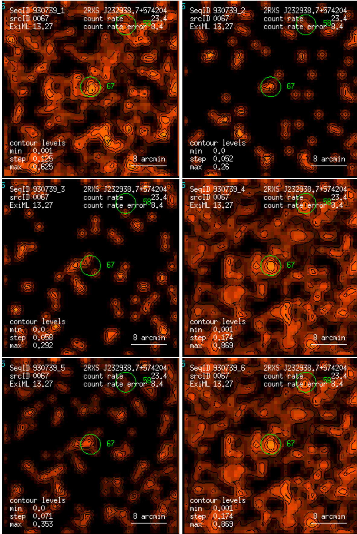
Figure 67: RASS 930739: detection 0067: band rate images, Gaussian filter: (1) PSPC channels 11 – 41, (2) 52 – 90, (3) 91 – 201, (4) 11 – 235, (5) 52 – 201, (6) 11 – 201. Broad band rates in counts/ks. Band rate contour levels in counts/ks/arcmin 2 .
