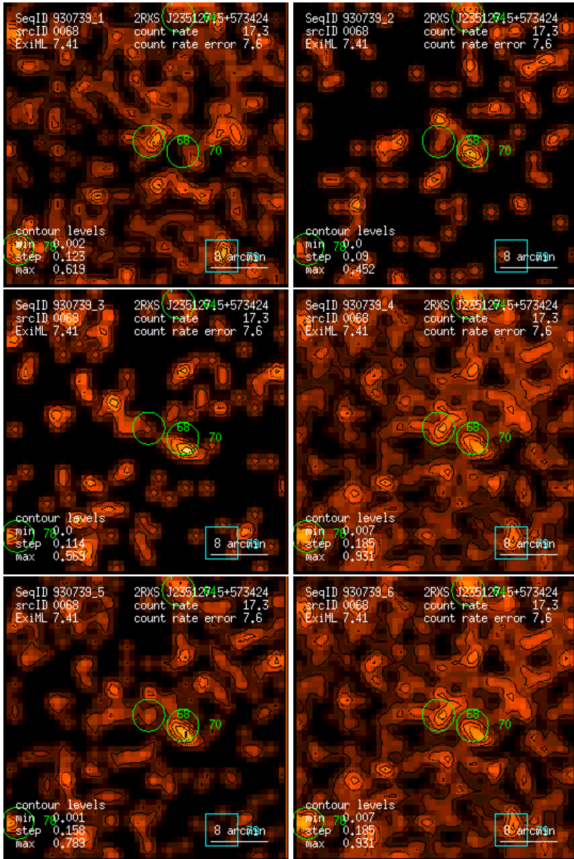
Figure 68: RASS 930739: detection 0068: band rate images, Gaussian filter: (1) PSPC channels 11 – 41, (2) 52 – 90, (3) 91 – 201, (4) 11 – 235, (5) 52 – 201, (6) 11 – 201. Broad band rates in counts/ks. Band rate contour levels in counts/ks/arcmin 2 .
