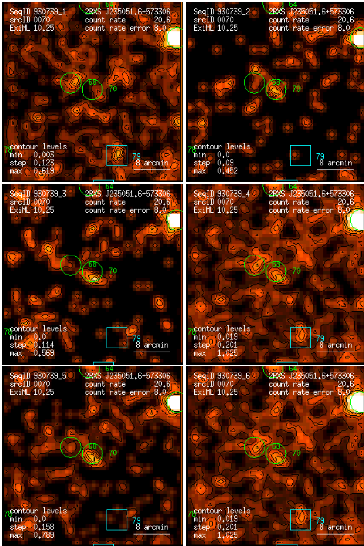
Figure 70: RASS 930739: detection 0070: band rate images, Gaussian filter: (1) PSPC channels 11 – 41, (2) 52 – 90, (3) 91 – 201, (4) 11 – 235, (5) 52 – 201, (6) 11 – 201. Broad band rates in counts/ks. Band rate contour levels in counts/ks/arcmin 2 .
