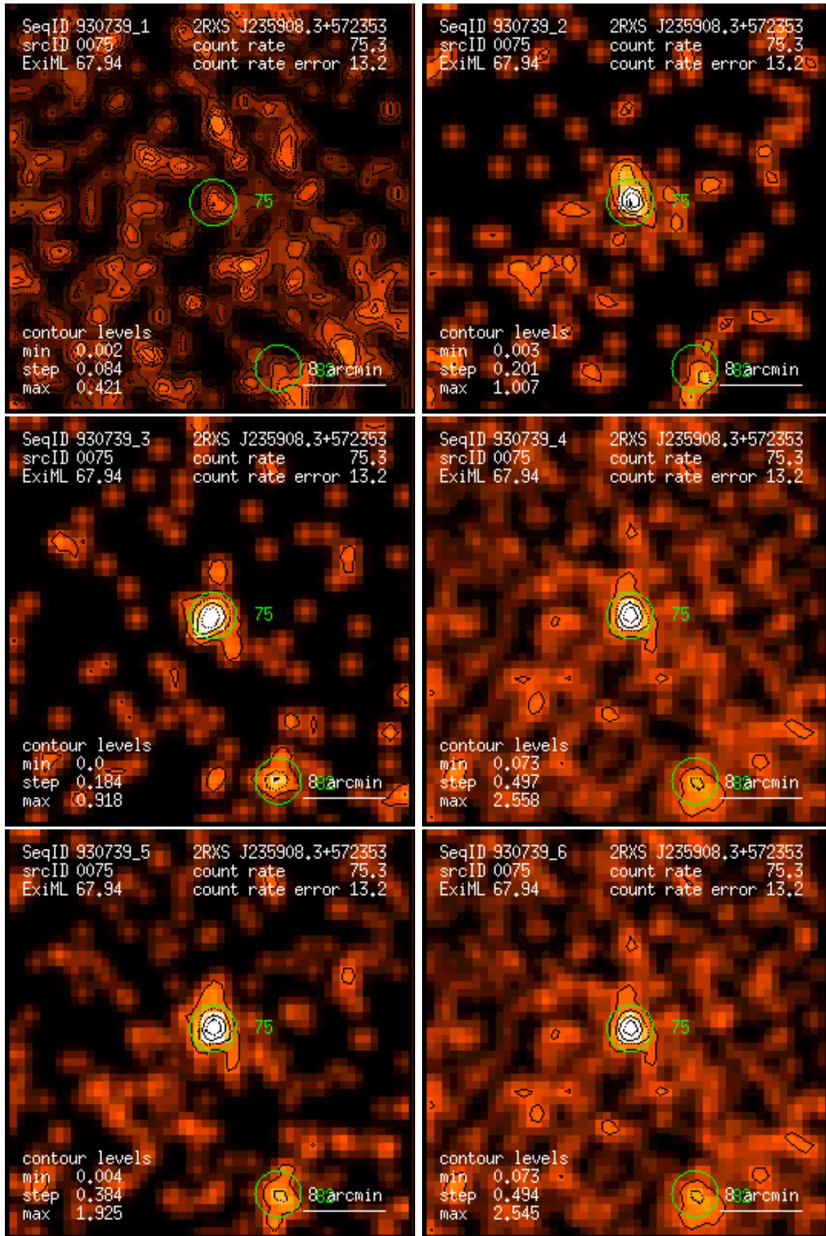
Figure 75: RASS 930739: detection 0075: band rate images, Gaussian filter: (1) PSPC channels 11 – 41, (2) 52 – 90, (3) 91 – 201, (4) 11 – 235, (5) 52 – 201, (6) 11 – 201. Broad band rates in counts/ks. Band rate contour levels in counts/ks/arcmin 2 .
