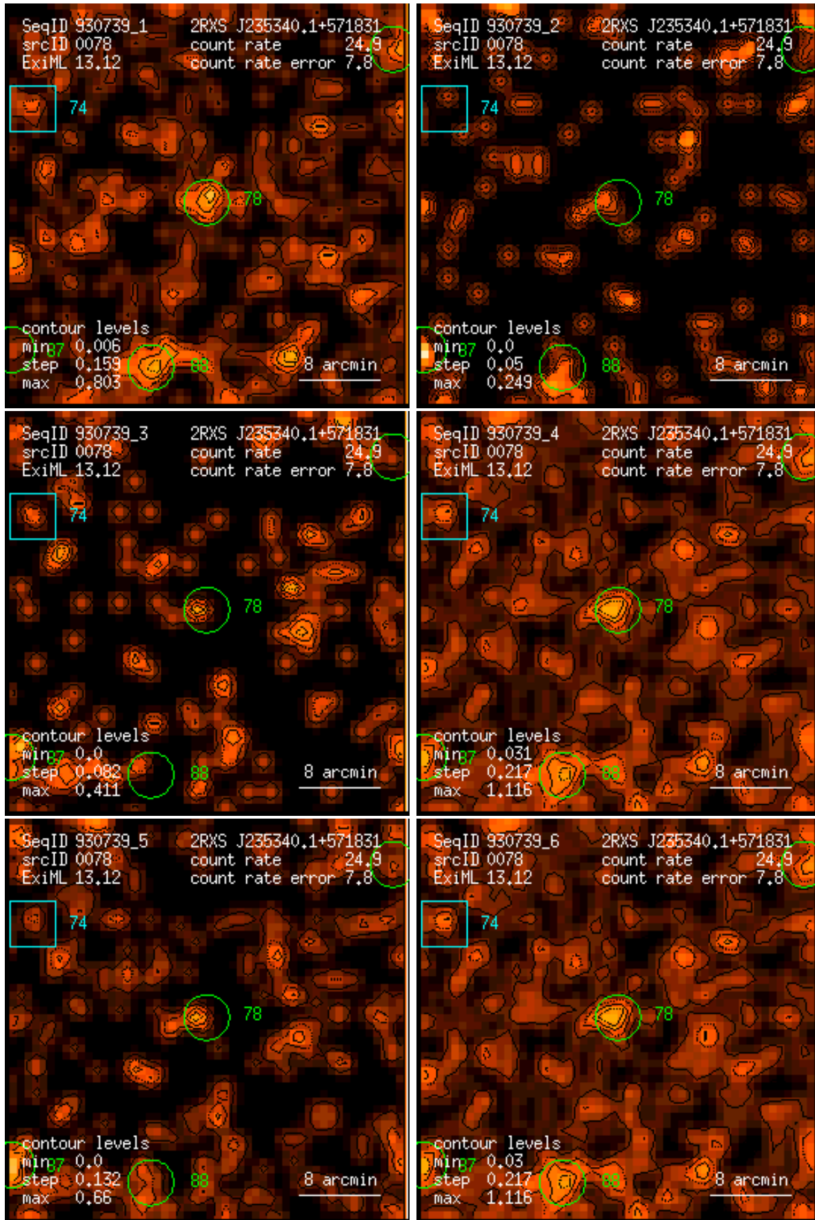
Figure 78: RASS 930739: detection 0078: band rate images, Gaussian filter: (1) PSPC channels 11 – 41, (2) 52 – 90, (3) 91 – 201, (4) 11 – 235, (5) 52 – 201, (6) 11 – 201. Broad band rates in counts/ks. Band rate contour levels in counts/ks/arcmin 2 .
