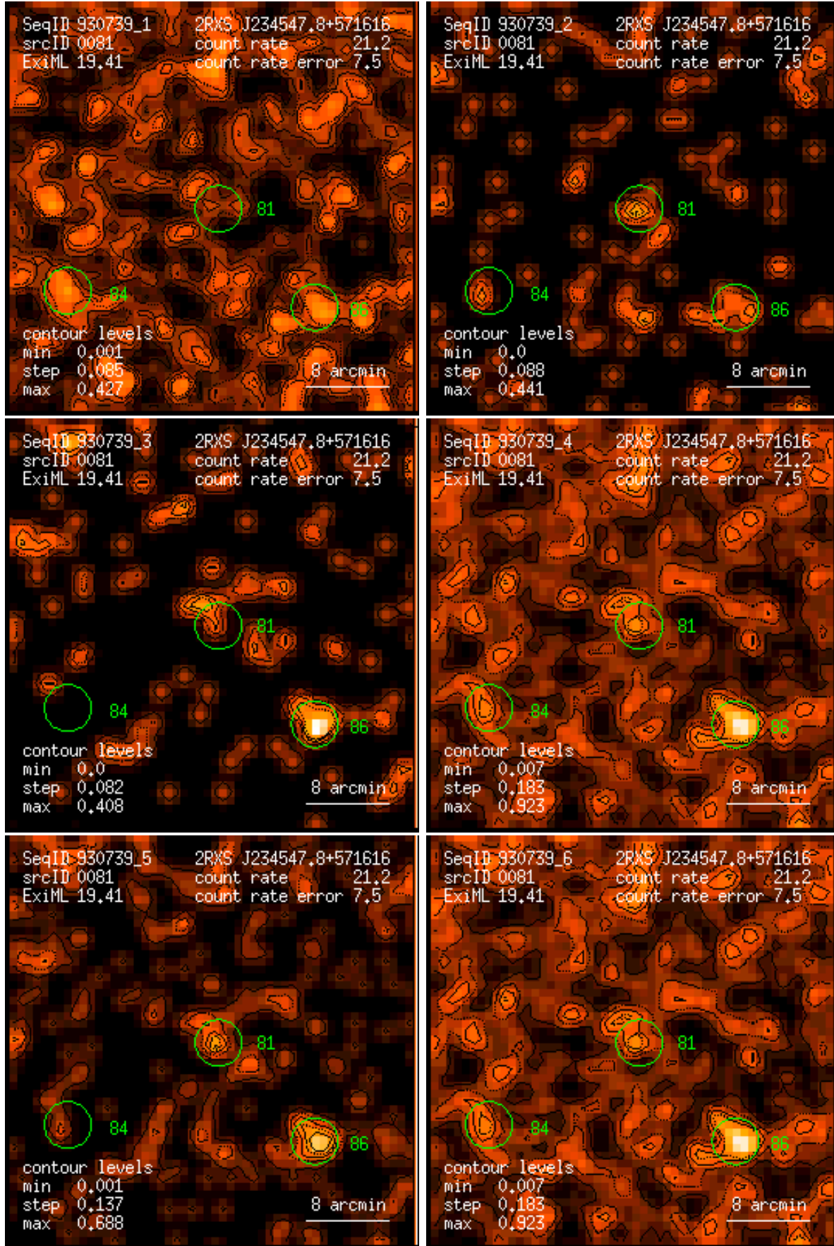
Figure 81: RASS 930739: detection 0081: band rate images, Gaussian filter: (1) PSPC channels 11 – 41, (2) 52 – 90, (3) 91 – 201, (4) 11 – 235, (5) 52 – 201, (6) 11 – 201. Broad band rates in counts/ks. Band rate contour levels in counts/ks/arcmin 2 .
