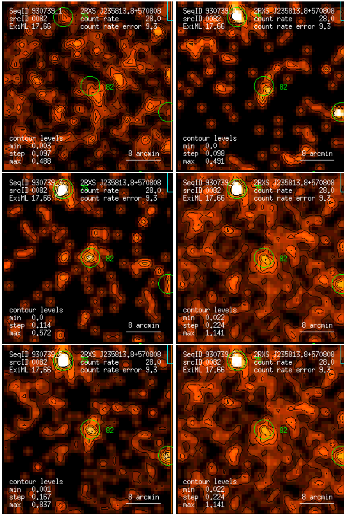
Figure 82: RASS 930739: detection 0082: band rate images, Gaussian filter: (1) PSPC channels 11 – 41, (2) 52 – 90, (3) 91 – 201, (4) 11 – 235, (5) 52 – 201, (6) 11 – 201. Broad band rates in counts/ks. Band rate contour levels in counts/ks/arcmin 2 .
