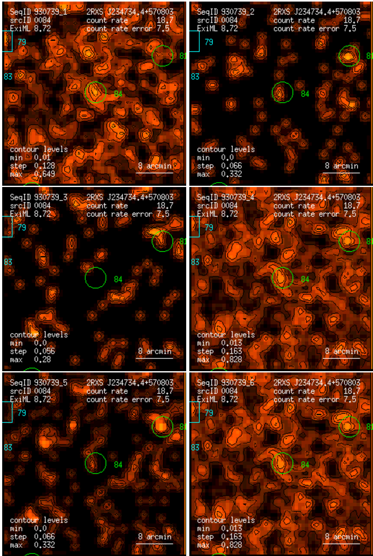
Figure 84: RASS 930739: detection 0084: band rate images, Gaussian filter: (1) PSPC channels 11 – 41, (2) 52 – 90, (3) 91 – 201, (4) 11 – 235, (5) 52 – 201, (6) 11 – 201. Broad band rates in counts/ks. Band rate contour levels in counts/ks/arcmin 2 .
